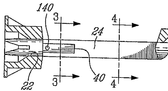
FIG-2 (Prior Art)
