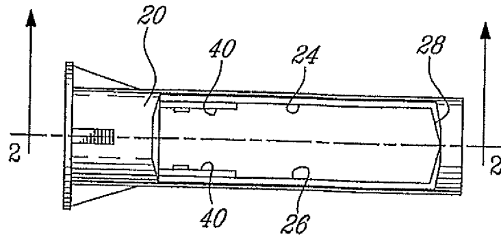
FIG-1 (Prior Art)
