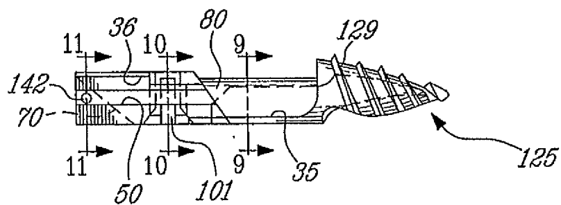
FIG-7 (Prior Art)
