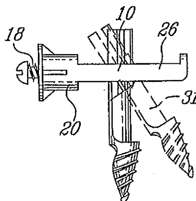
FIG-14 (Prior Art)
