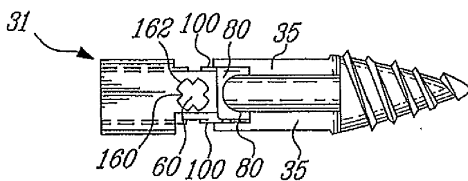
FIG-6 (Prior Art)
