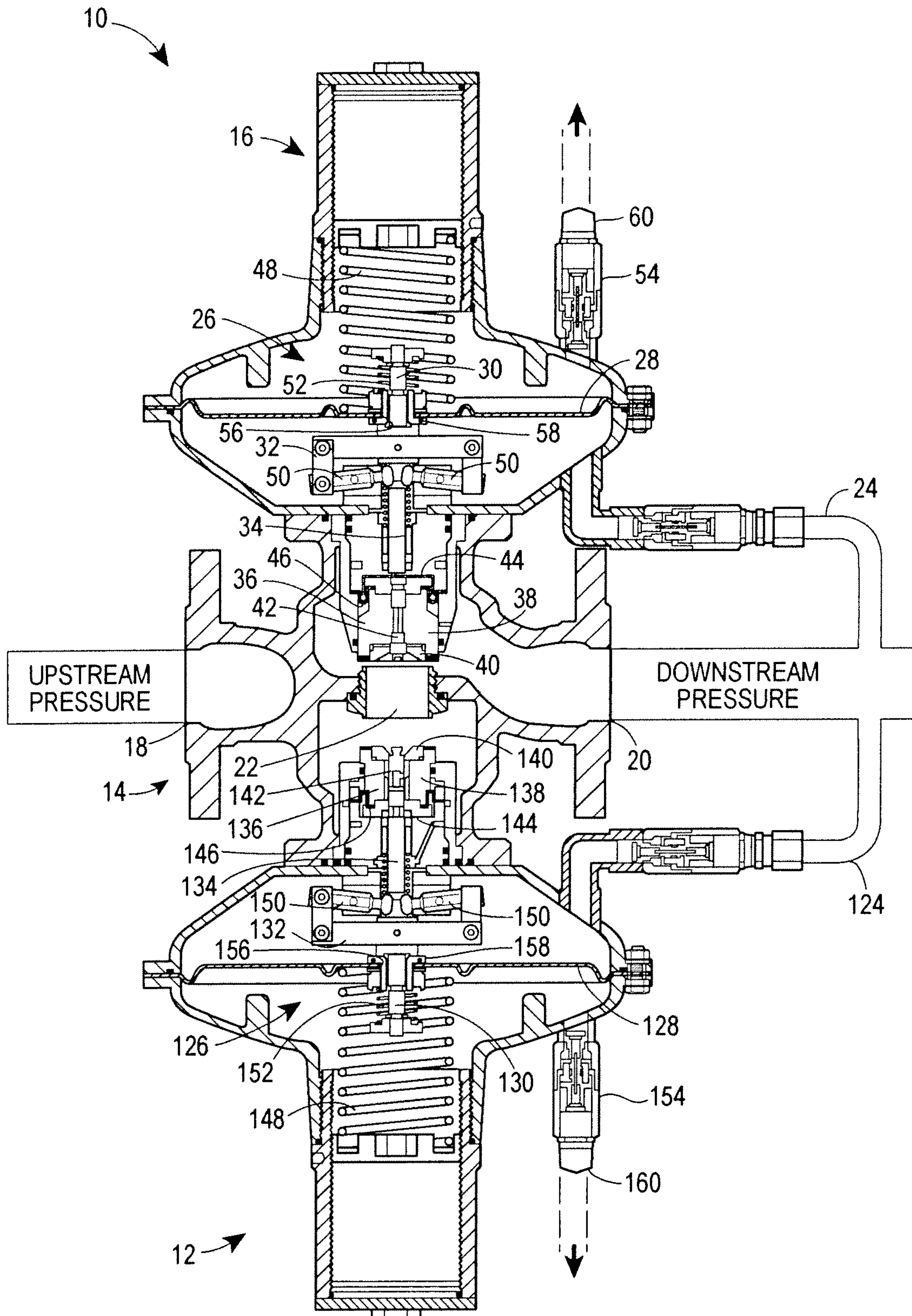
FIG. 1 PRIOR ART
