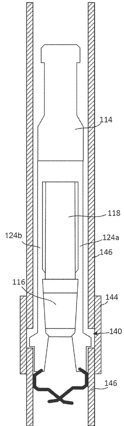
Fig. 2D (Prior Art)
