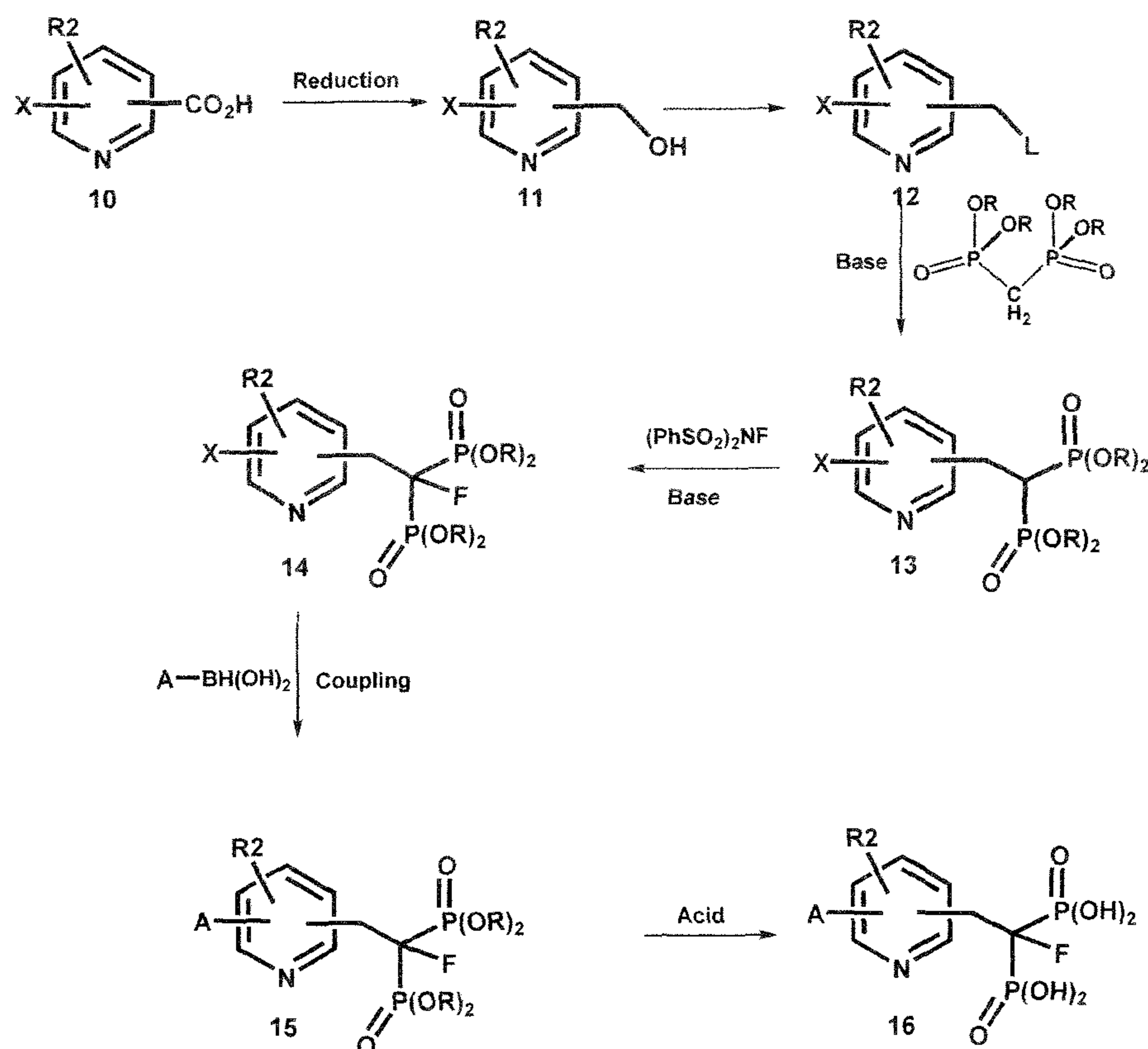
Scheme 2: General synthesis of pyridinyl fluoroethanyl bisphosphonate analogs
