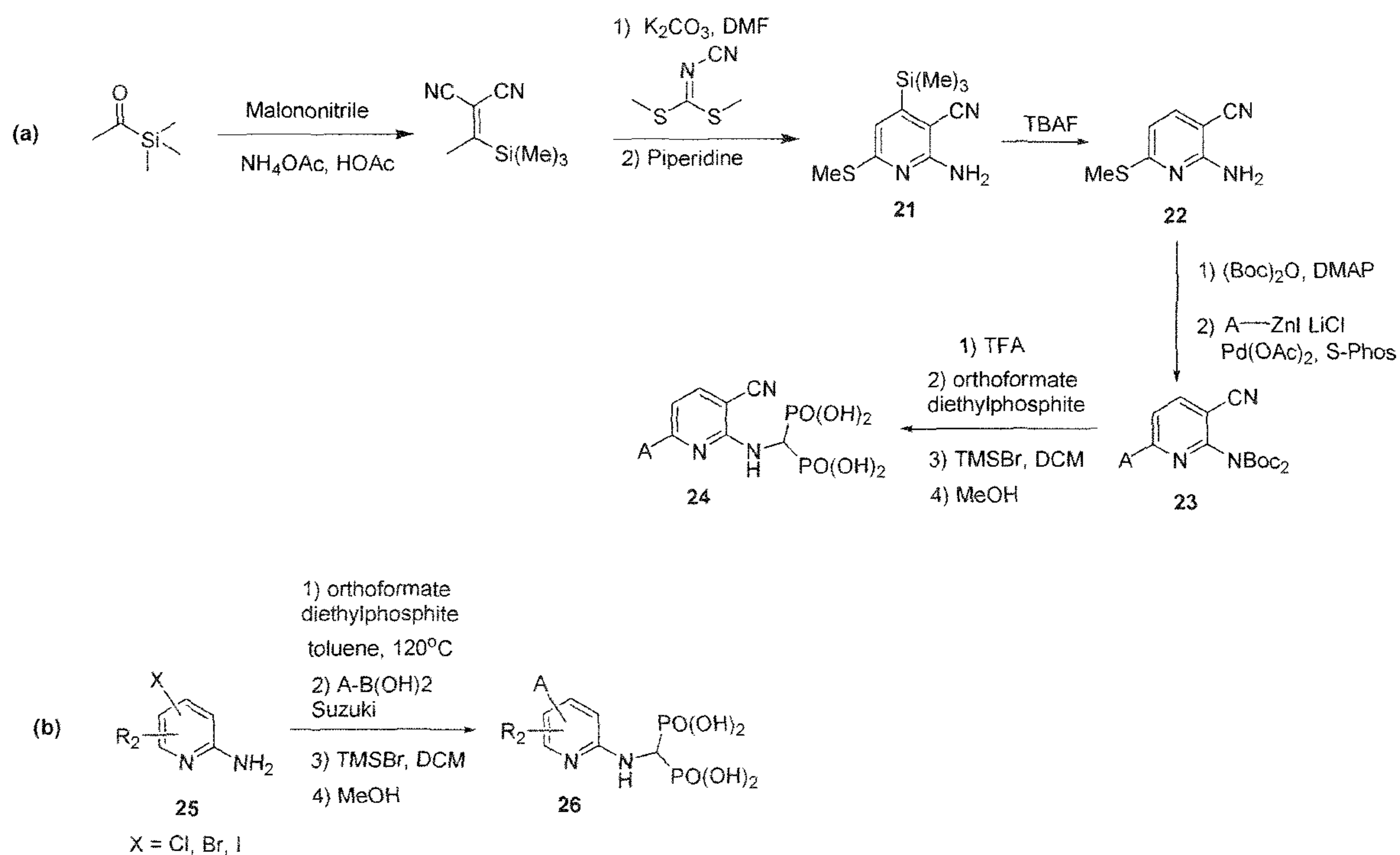
Scheme 3: General synthesis of pyridinylamino bisphosphonate analogs
