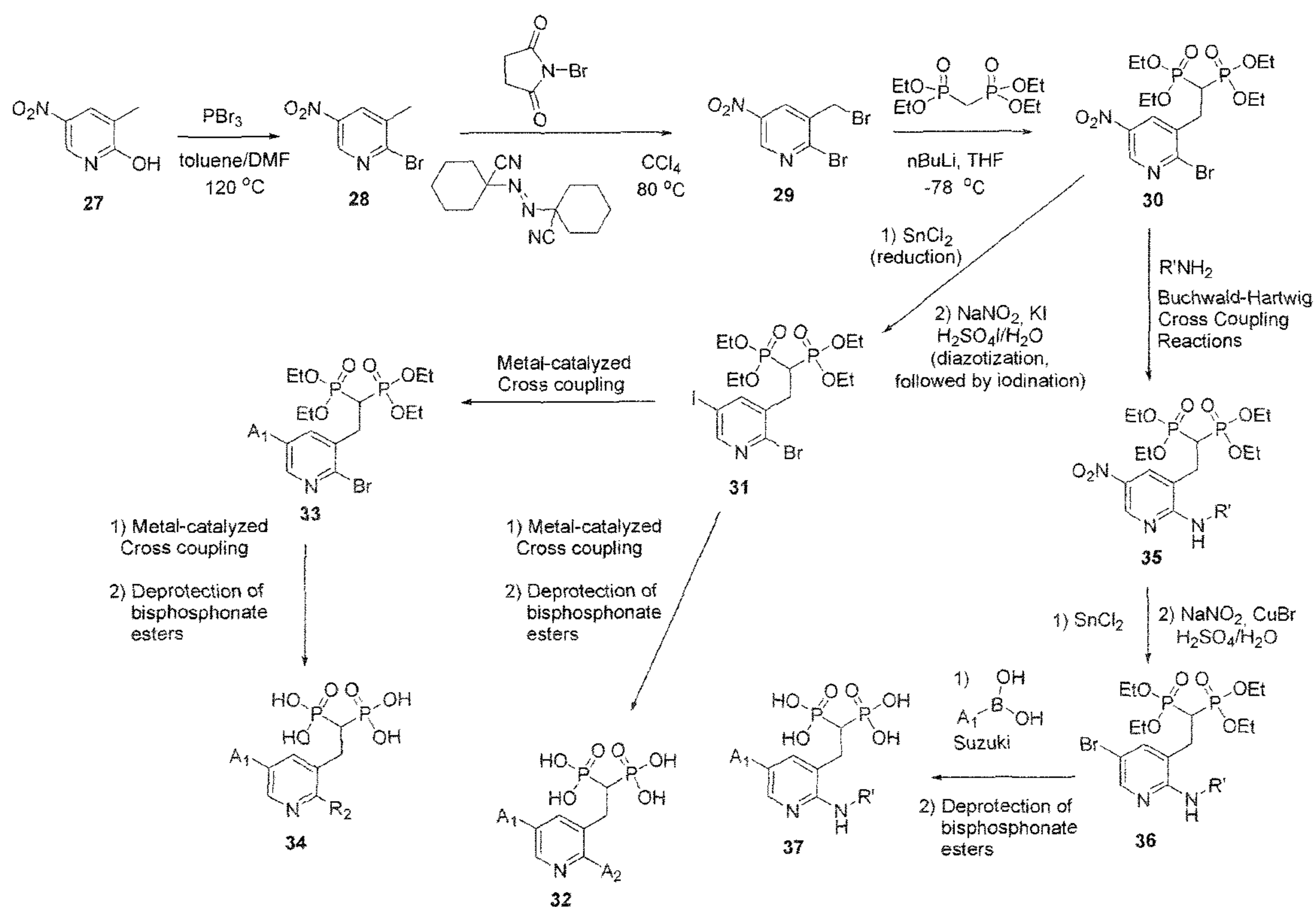
Scheme 4: General synthesis of selectively branched pyridinyl bisphosphonate analogs
