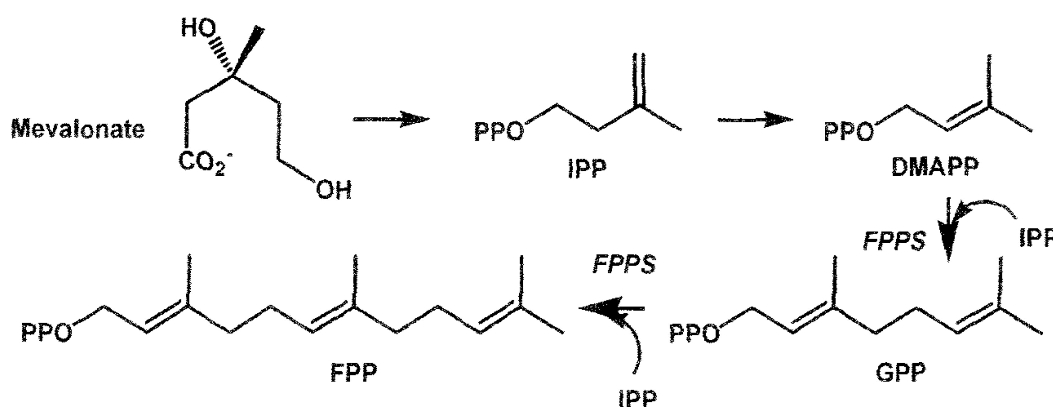
Scheme 1: Pathway of human farnesyl pyrophosphate
