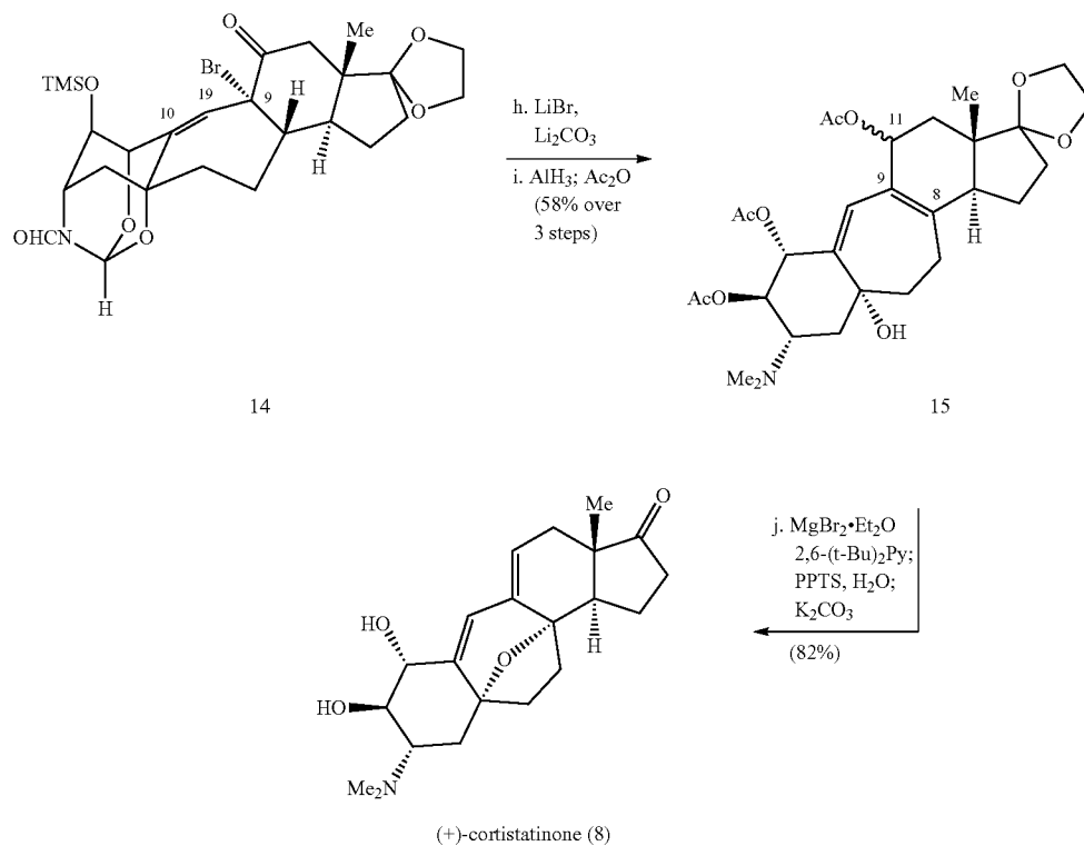
Scheme 5
