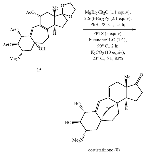
Cortistatinone Compound 8:
