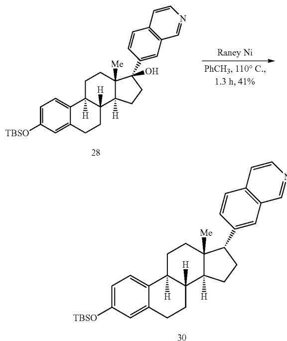
17- \alpha -isoquinoline estrone Compound 30:
