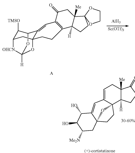
Alternative Synthesis of Cortistatinone Compound 8
