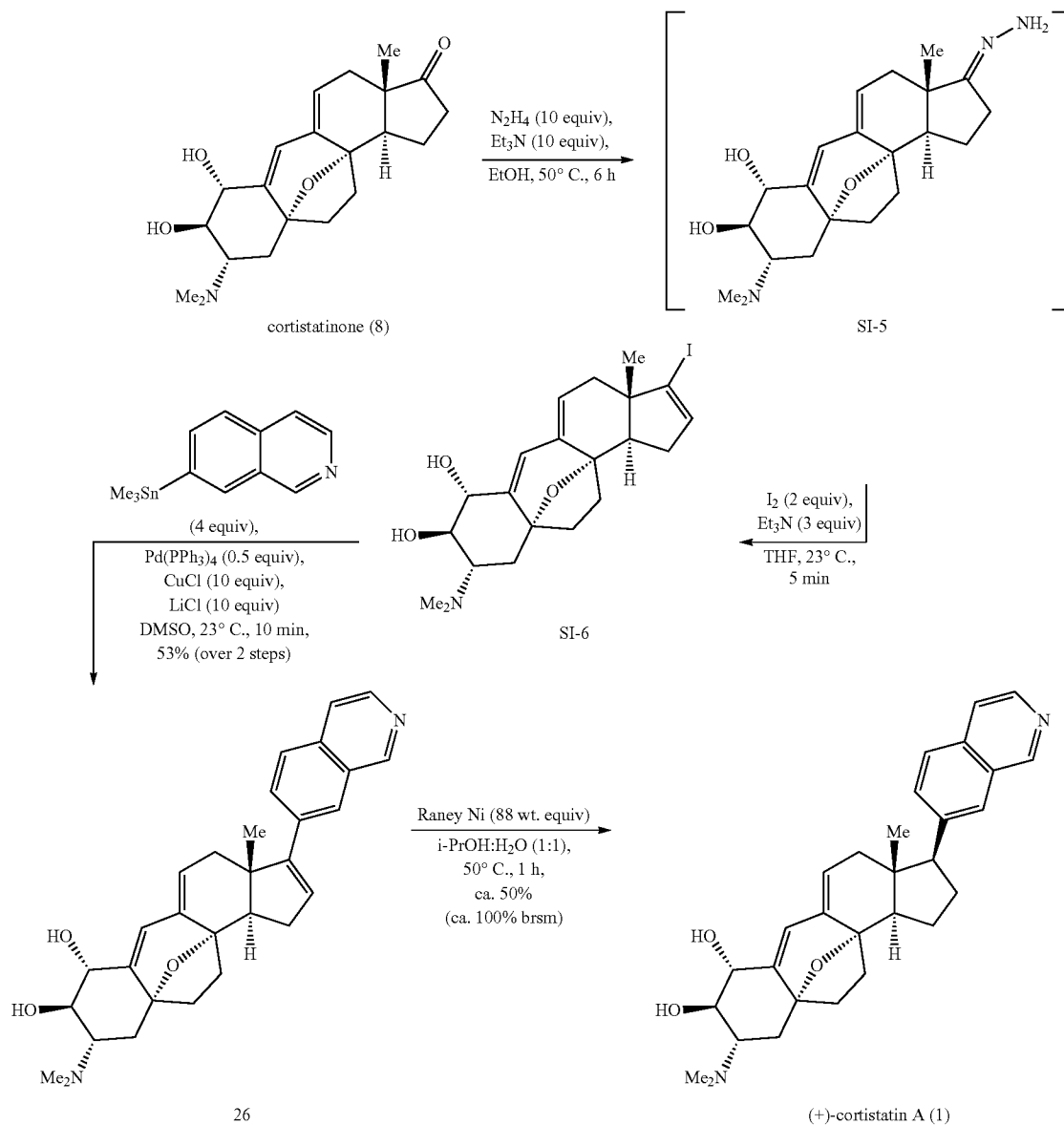
Scheme 7
