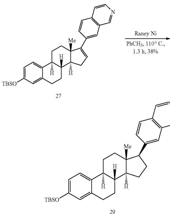
17- \beta -isoquinoline estrone Compound 29:
