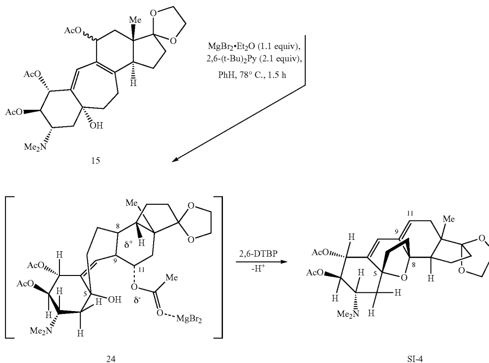
Scheme 6A
