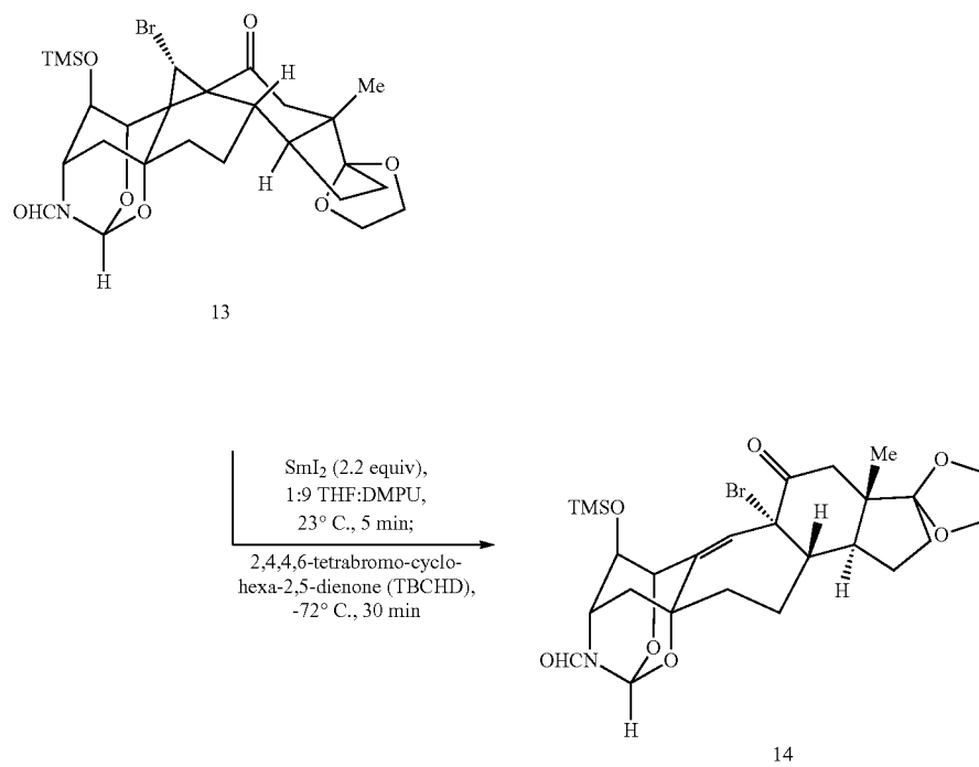
Scheme 5A
