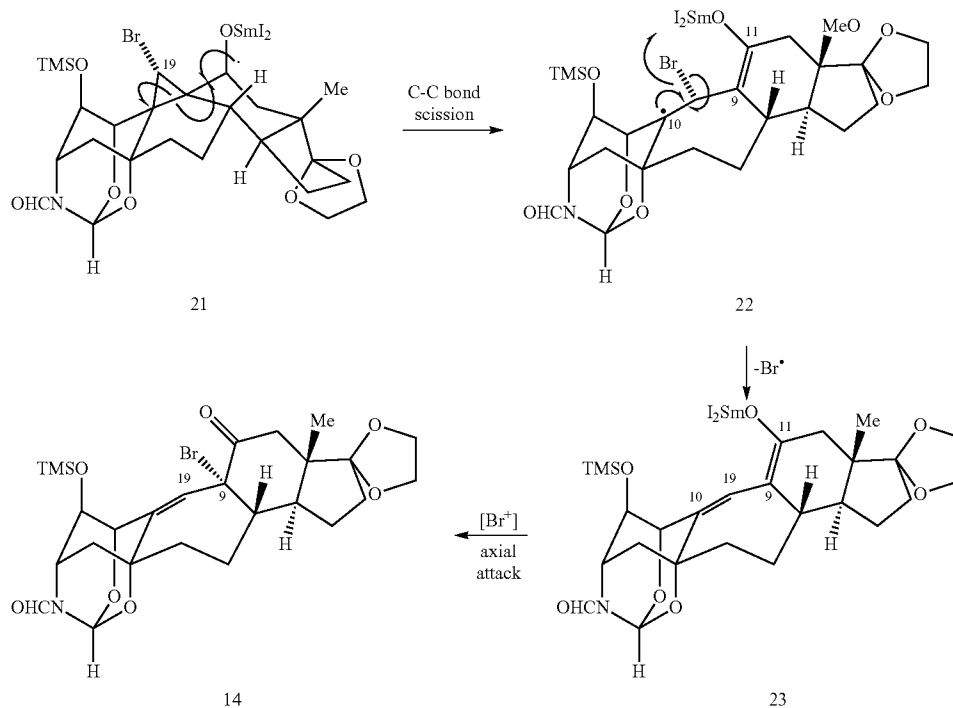
Scheme 4
