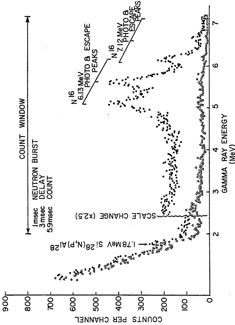
OXYGEN ACTIVATION SPECTRA PULSED MODE OPERATION
