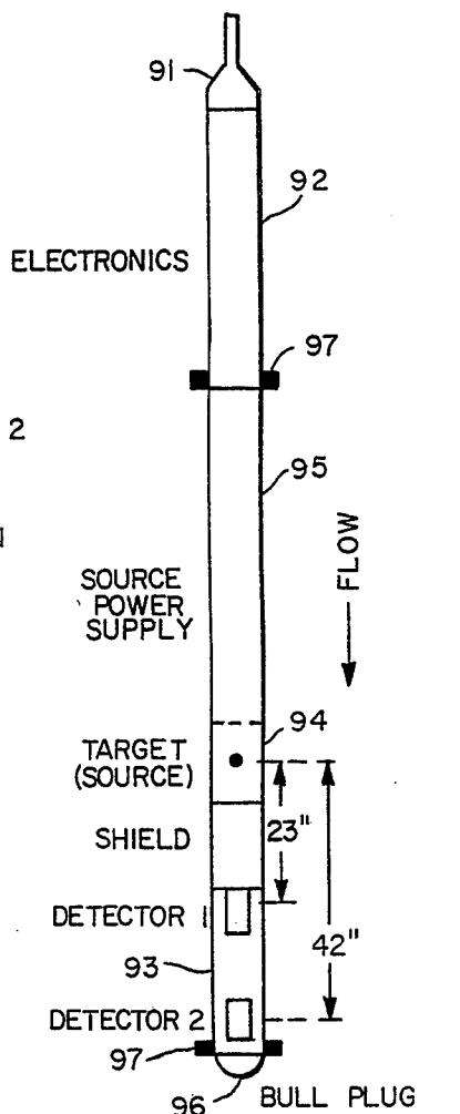
ASSEMBLY FOR WATER FLOWING DOWN
