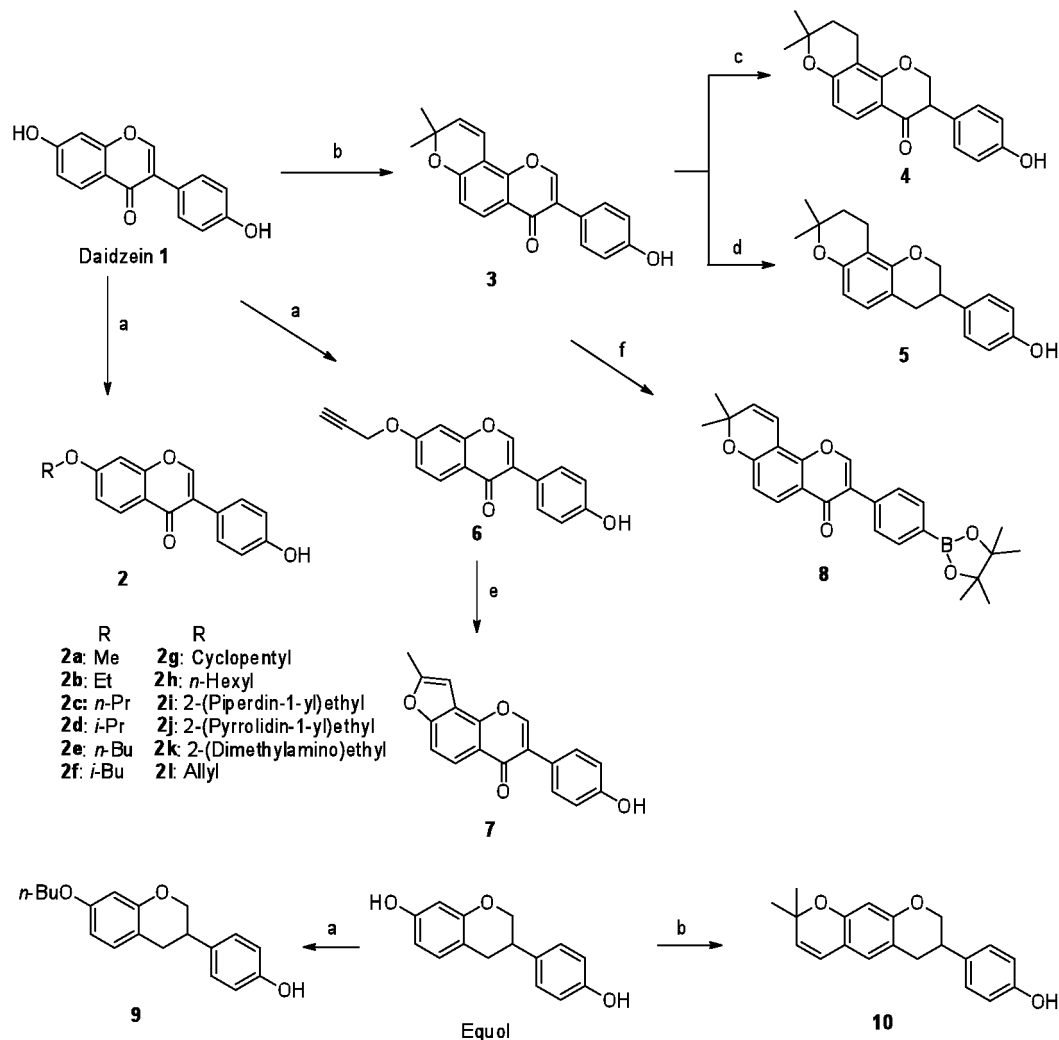
[0125] Scheme 1 Synthesis of daidzein derivatives and analogs. Reagents and conditions: (a) K 2 CO 3 , DMSO, RBr or RCl, rt; (b) xylene, 130°C, microwave; (c) H 2 , 10% Pd/C, ethyl acetate, rt; (d) H 2 , 10% Pd/C, MeOH, rt; (e) CsF, N,N -diethylaniline, 130°C; (f) i). (CF 3 SO 2 ) 2 O, pyridine, CH 2 Cl 2 , 0°C - rt; ii).
