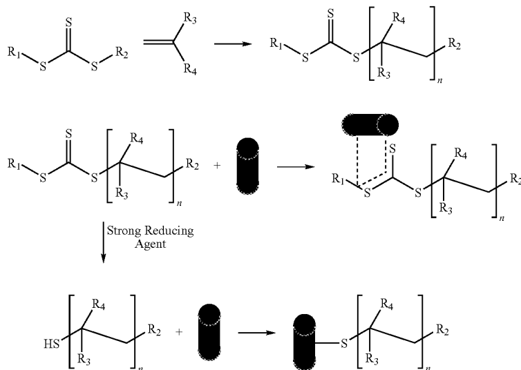
Scheme 2
