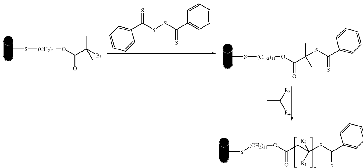
Scheme 6
