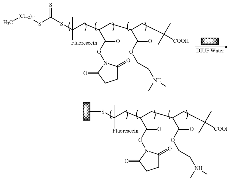
Scheme 4
