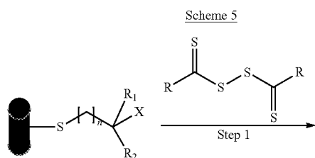
Scheme 5
