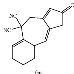
Terpenoid scaffold
