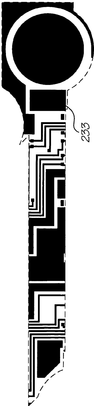
Metal 2 mask
