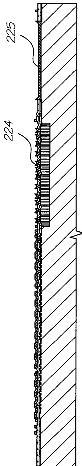
Deposit Metal 1
