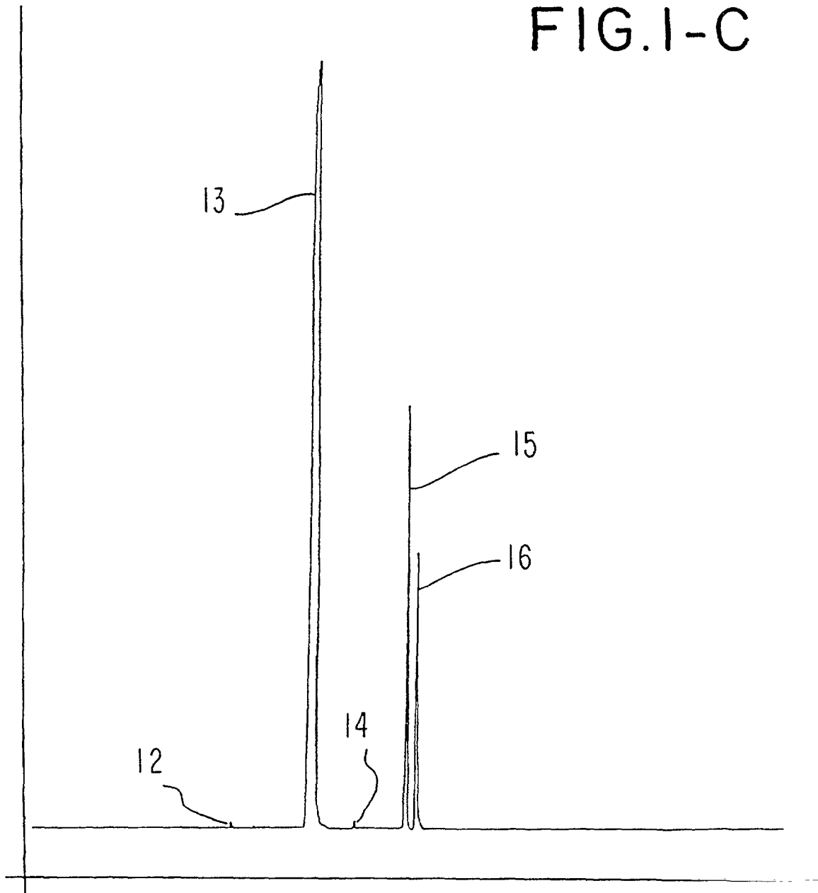
TOTAL ION CHROMATOGRAM FOR EXAMPLE I.
