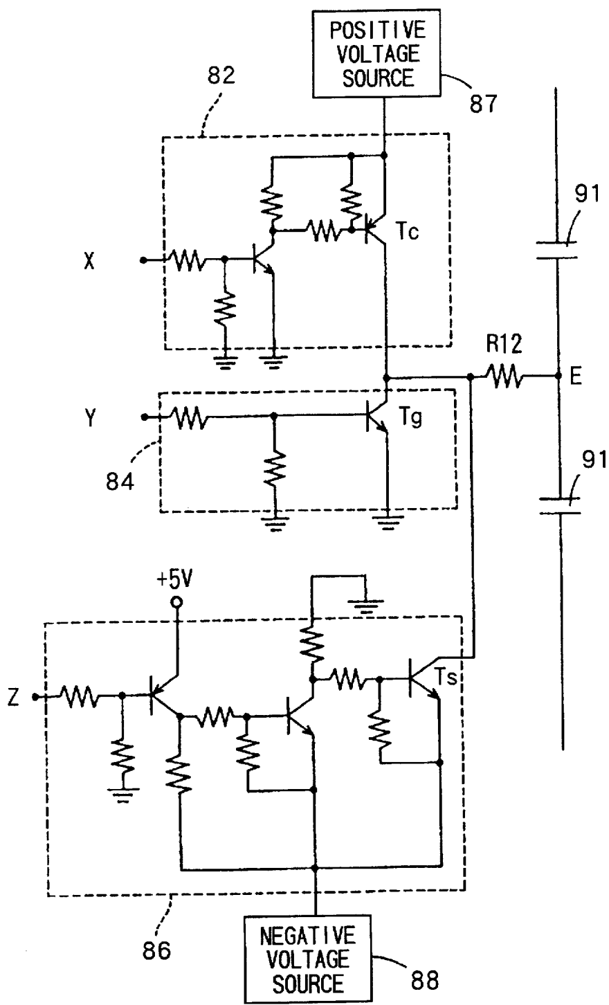
FIG. 7 PRIOR ART
