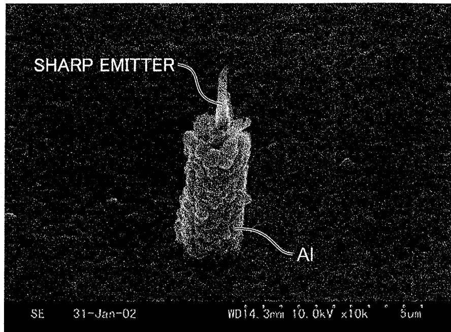
SHARP EMITTER WITH AN AL ELECTRODE
