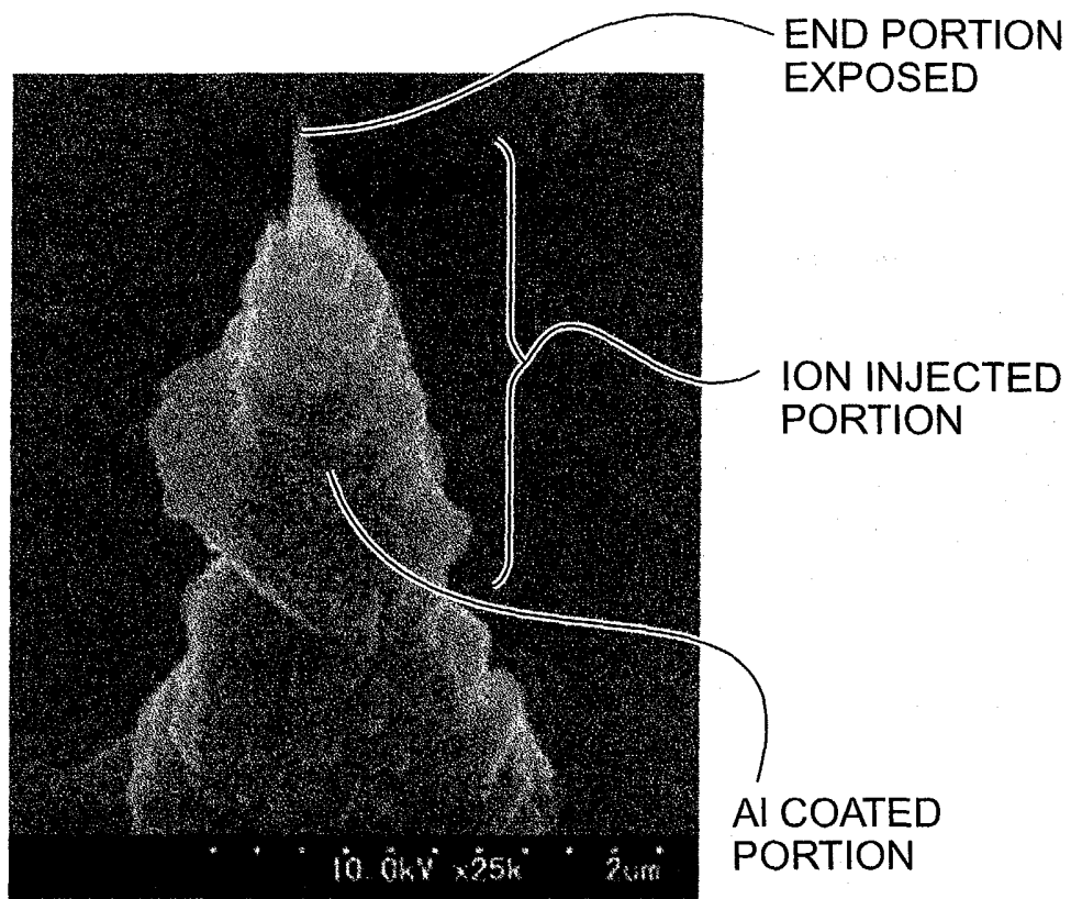
PROTRUSION WHERE AN AI ELECTRODE IS FORMED EXCEPT FOR THE TIP
