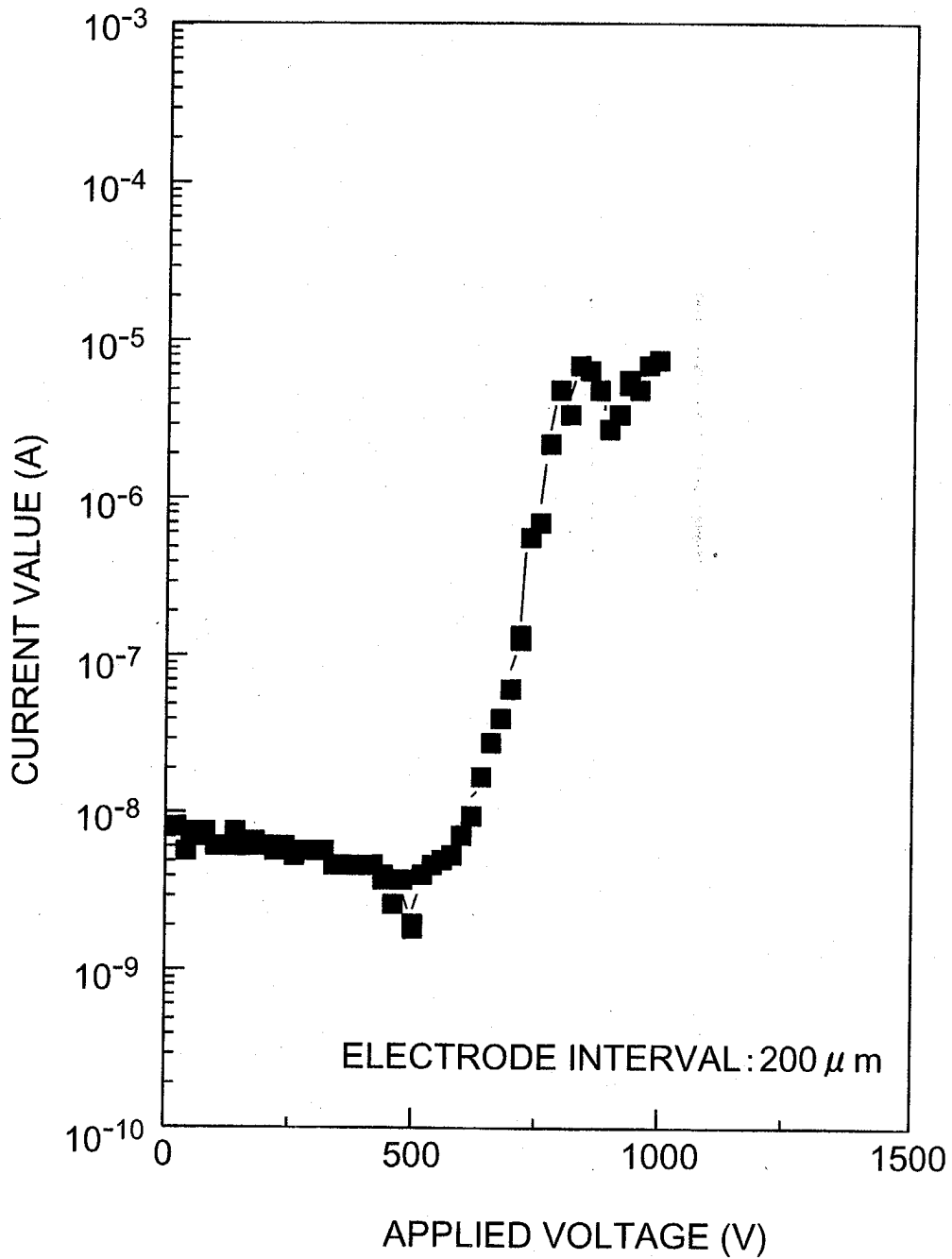
ELECTRON EMISSION CHARACTERISTIC OF A SHARP EMITTER INCLUDING A BORON DOPED EXITAXIAL LAYER AND BEING PROVIDED WITH AN AL ELECTRODE
