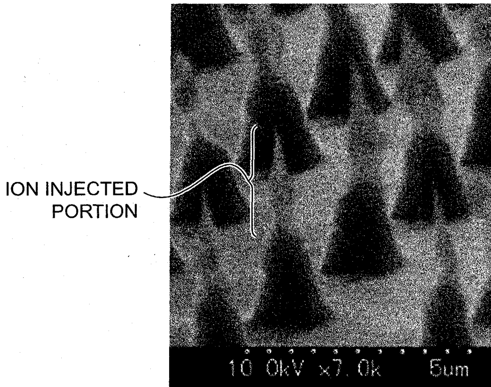
SHARP EMITTER WITH AN Al ION INJECTED LAYER
