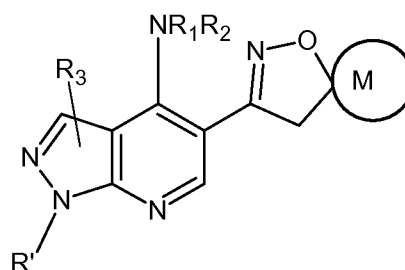
Formula XXXVI
