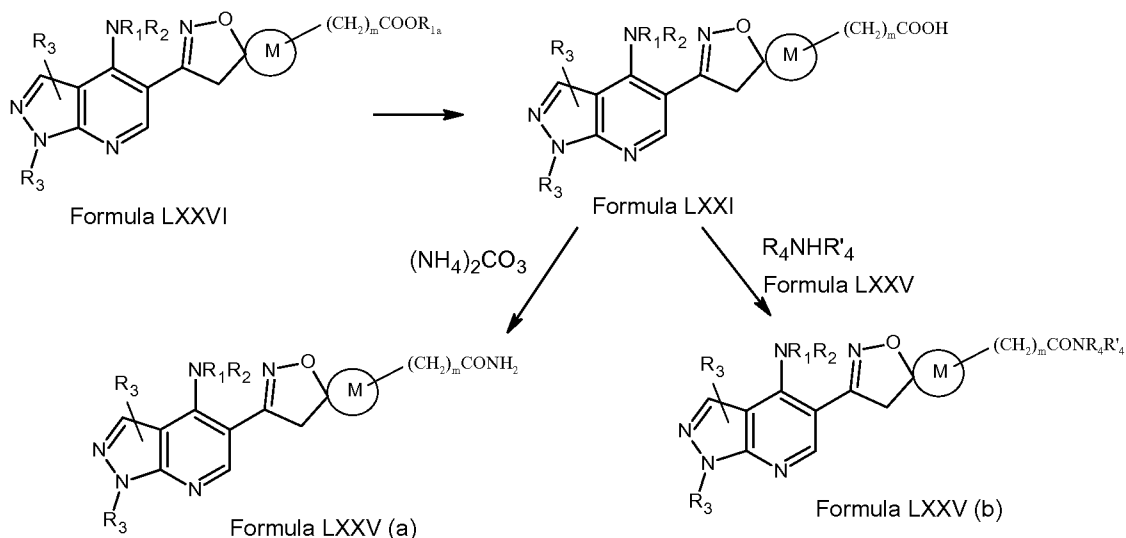
Scheme XIV
