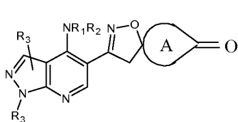
Formula XXXIII
