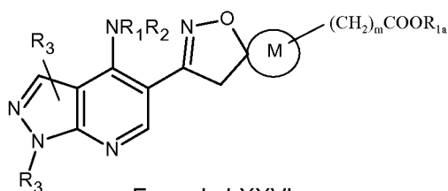
Formula LXXVI
