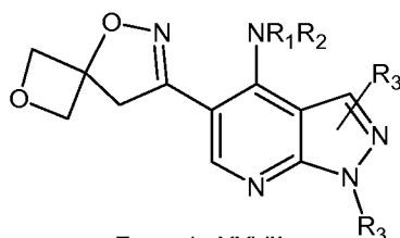
Formula XXVII
