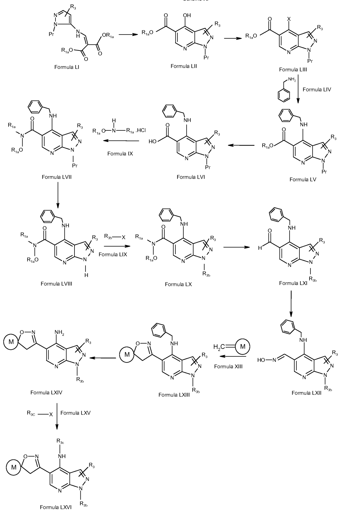
Scheme XI
