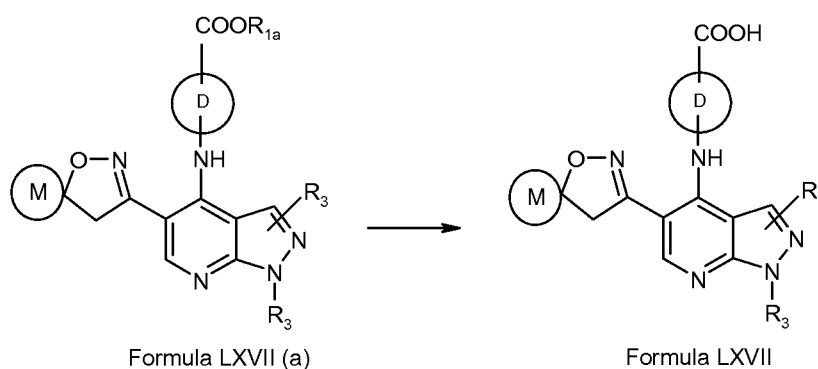
Scheme XII
