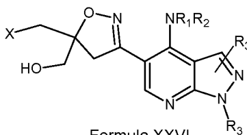
Formula XXVI
