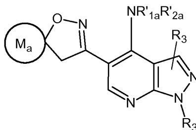
8 Formula Ia
