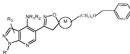
Formula XLII
