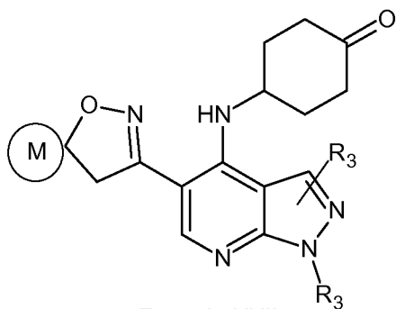
Formula XXII
