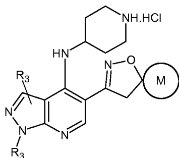
Formula XXXVIII
