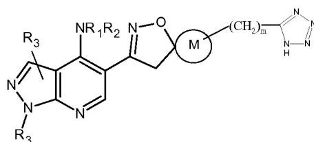
Formula LXXII
