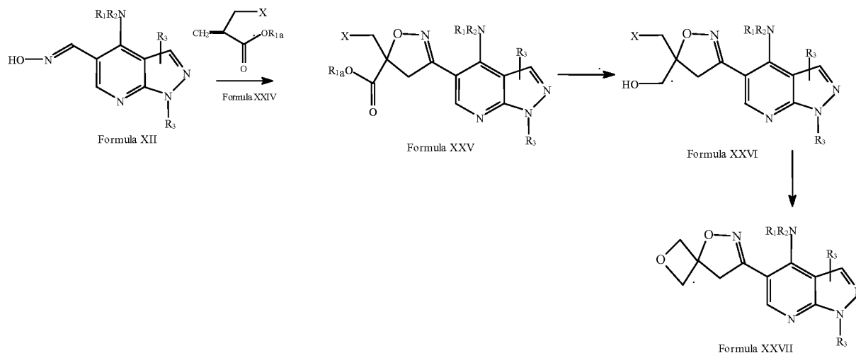
Scheme IV
