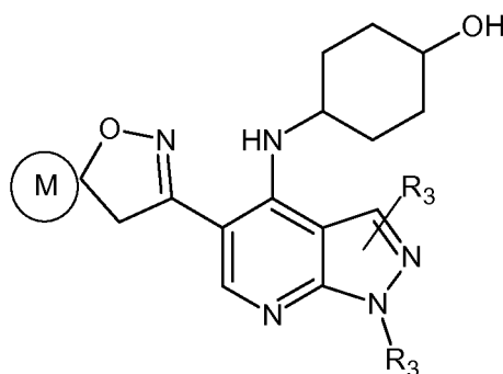
Formula XXI
