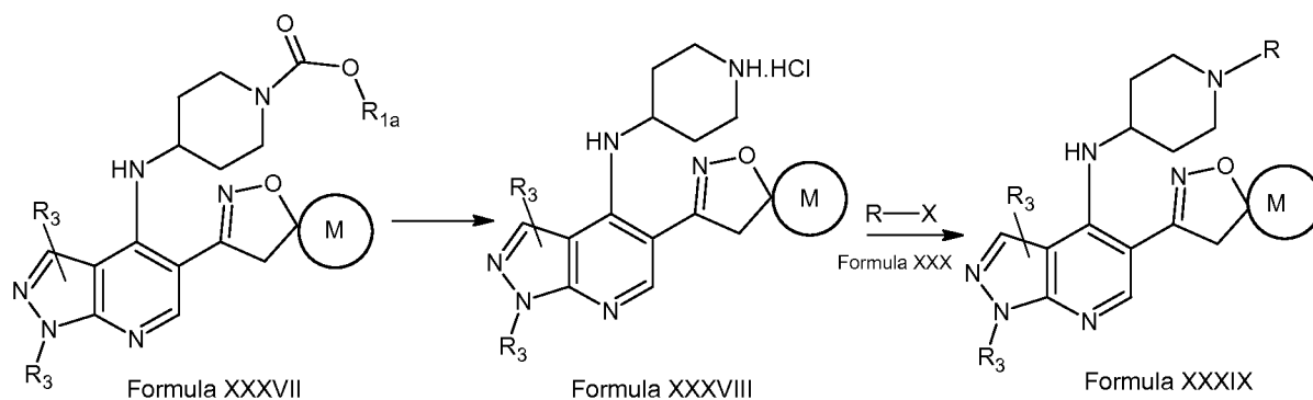
Scheme VIII
