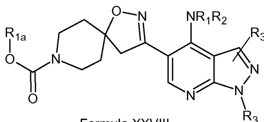
Formula XXVIII
