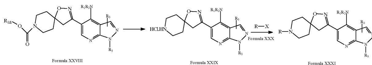
Scheme V
