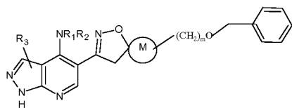
Formula XLI
