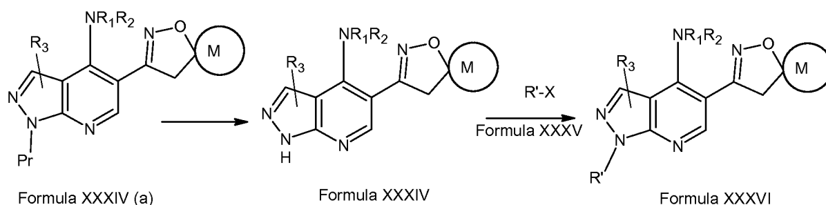
Scheme VII
