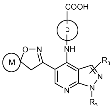
Formula LXVII
