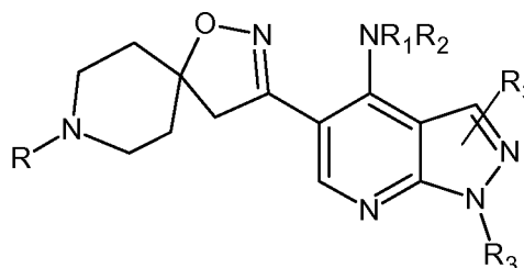
Formula XXXI
