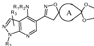
Formula XXXII
