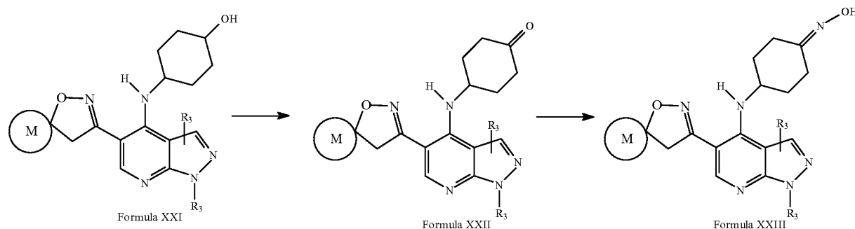
Scheme III
