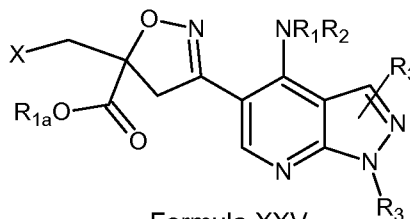
Formula XXV
