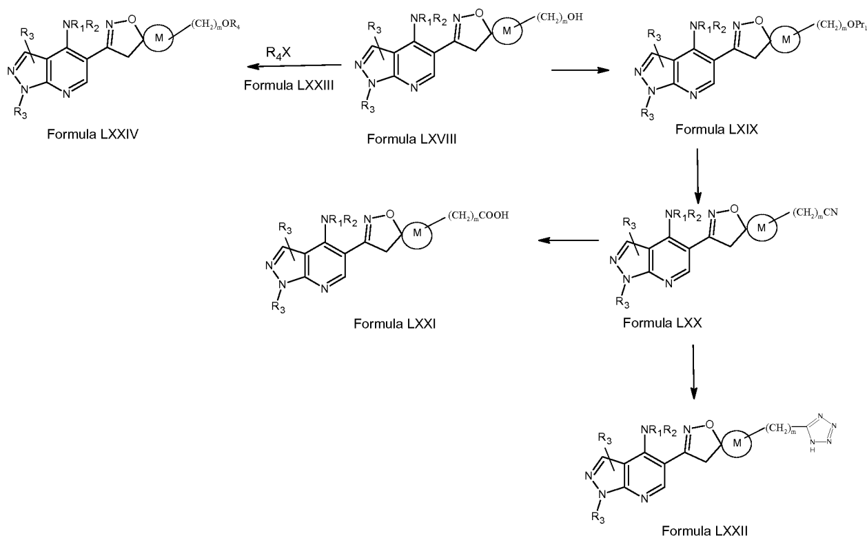
Scheme XIII
