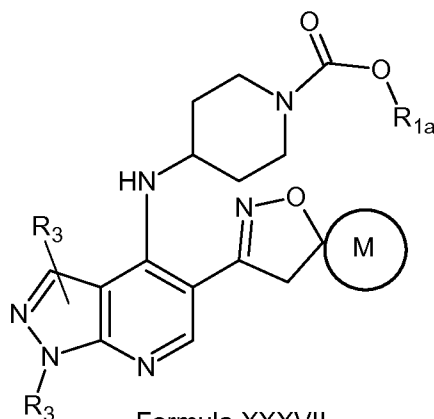
Formula XXXVII
