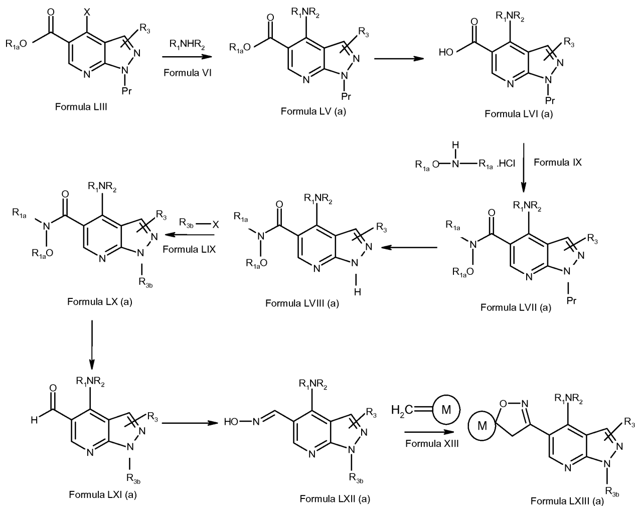
Scheme XI a
