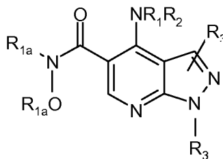
Formula X
