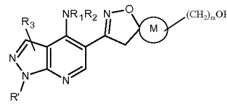
Formula XLIII
