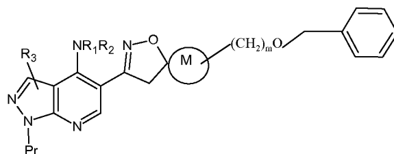
Formula XL
