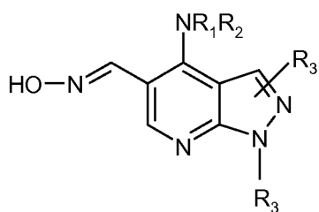
Formula XII
