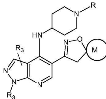
Formula XXXIX
