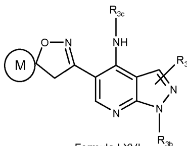
Formula LXVI
