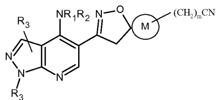
Formula LXX
