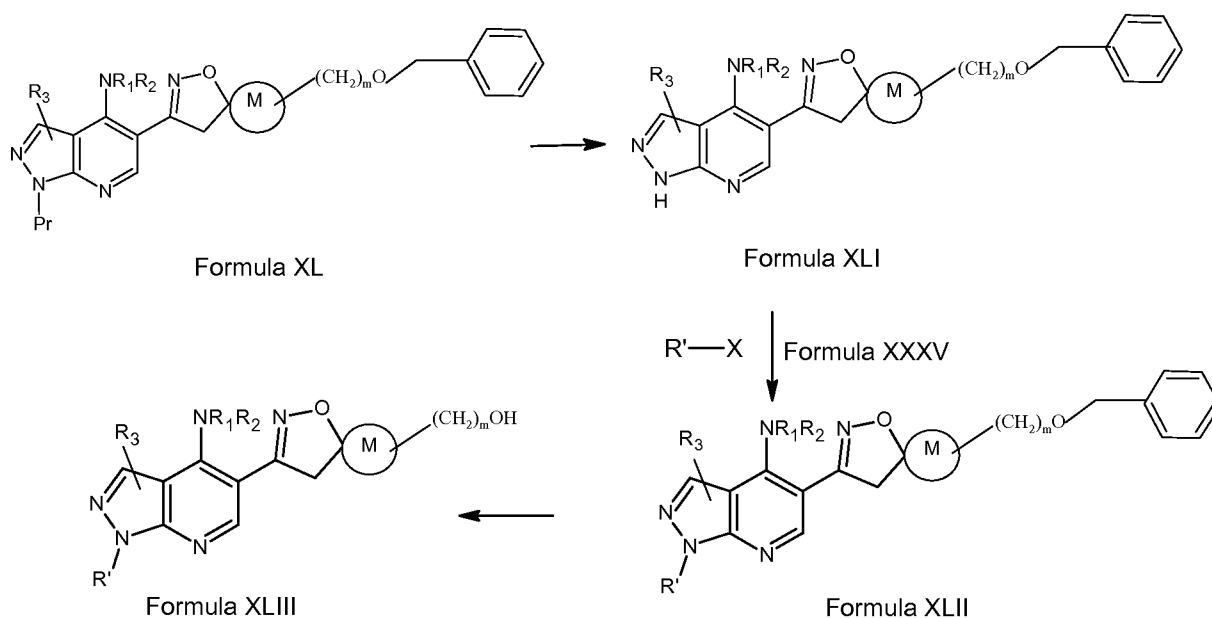
Scheme IX
