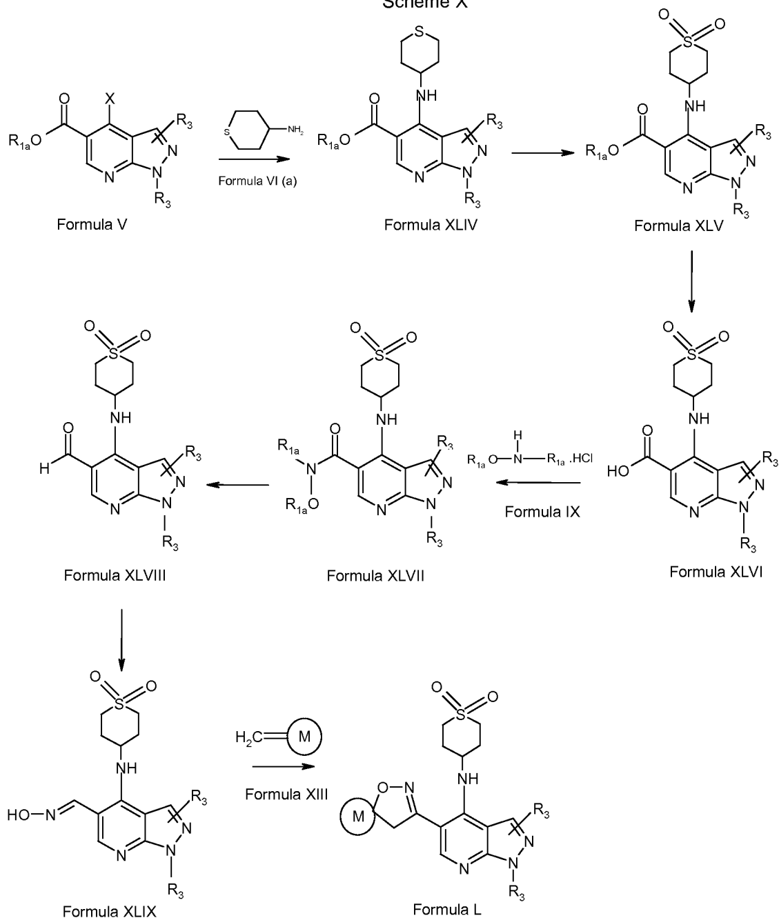
Scheme X
