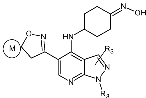
Formula XXIII
