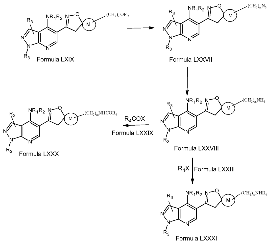
Scheme XV
