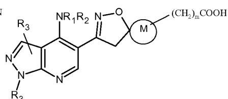
Formula LXXI
