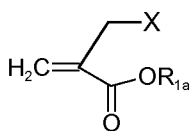
Formula XXIV
