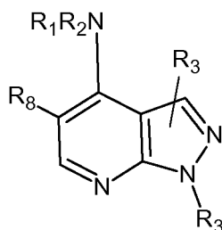
Formula Ib
