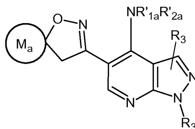
Formula Ia
