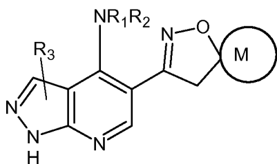
Formula XXXIV
