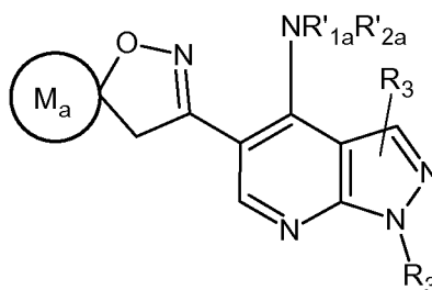
Formula Ia
