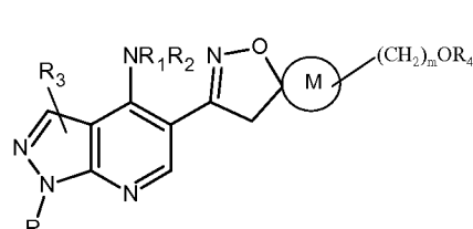
Formula LXXIV
