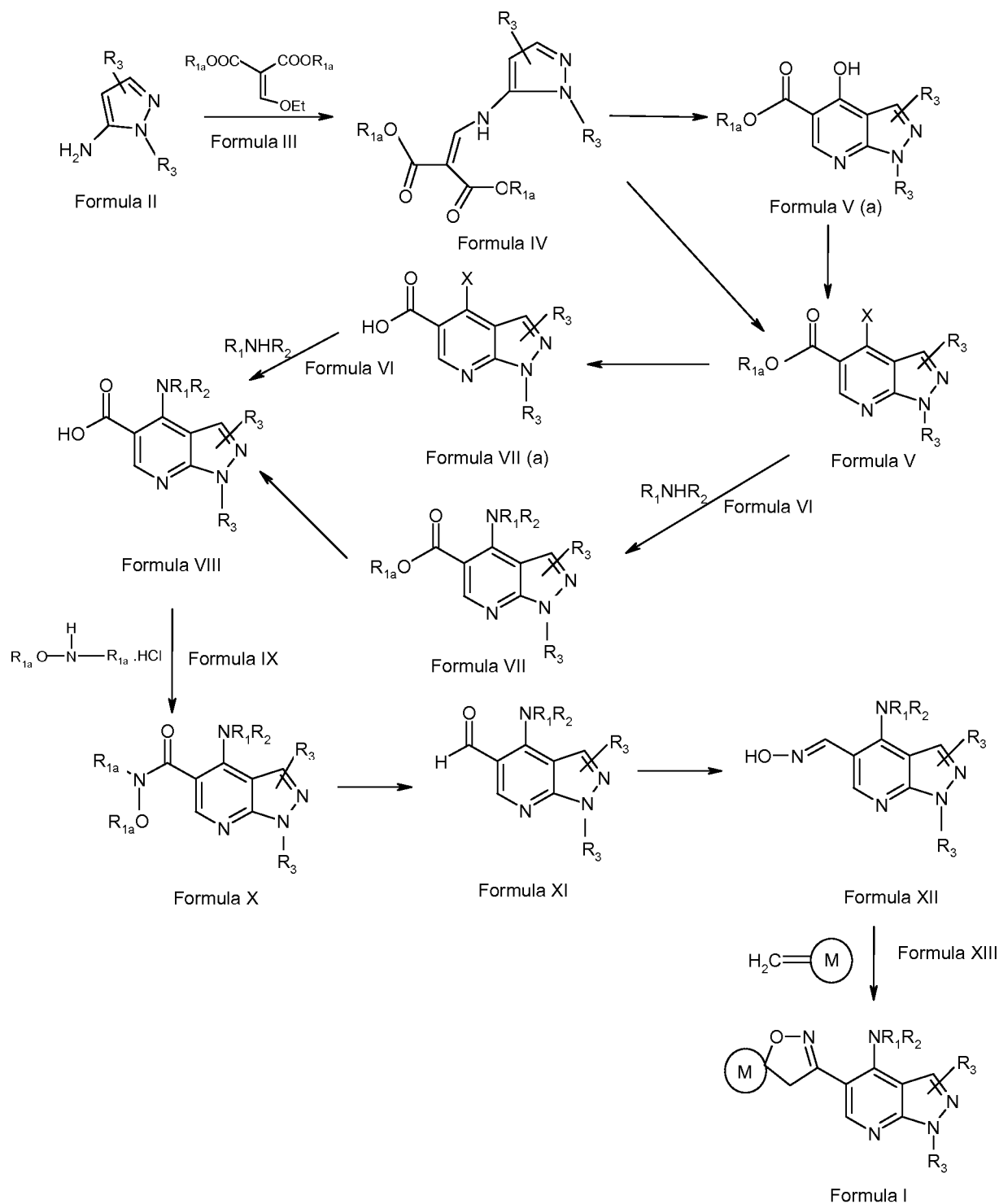
Scheme I
