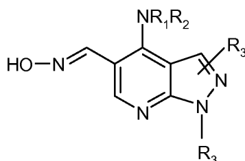
Formula XII
