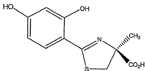
(S)-4'-(HO)-DADFT
