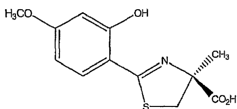
(S)-4'-(CH 3 O)-DADFT
