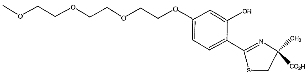
(S)-4'-(HO)-DADFT-PE
