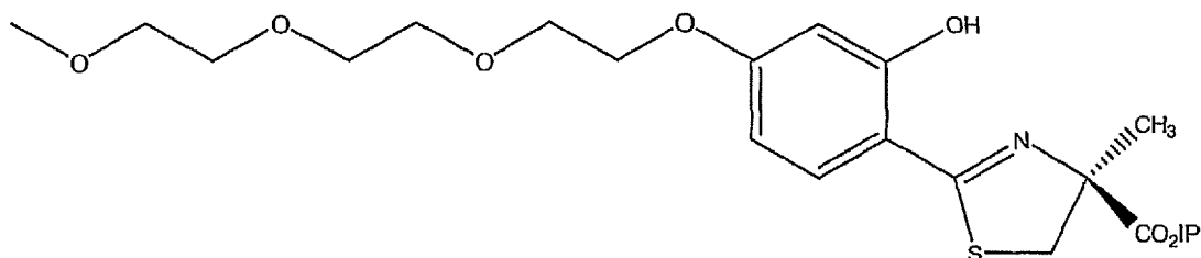
(S)-4'-(HO)-DADFT-PE iPrE
