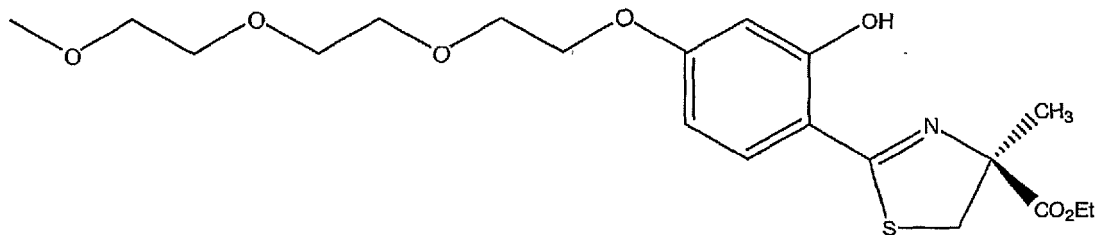
(S)-4'-(HO)-DADFT-PE EE
