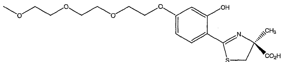
(S)-4'-(HO)-DADFT-PE
