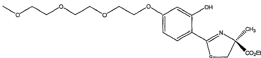
(S)-4'-(HO)-DADFT-PE-EE
