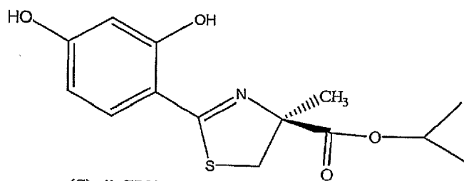
(S)-4'-(HO)-DADFT-iPrE
