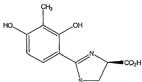
(S)-3'-(CH 3 )-4'-(HO)-DADMDFT
