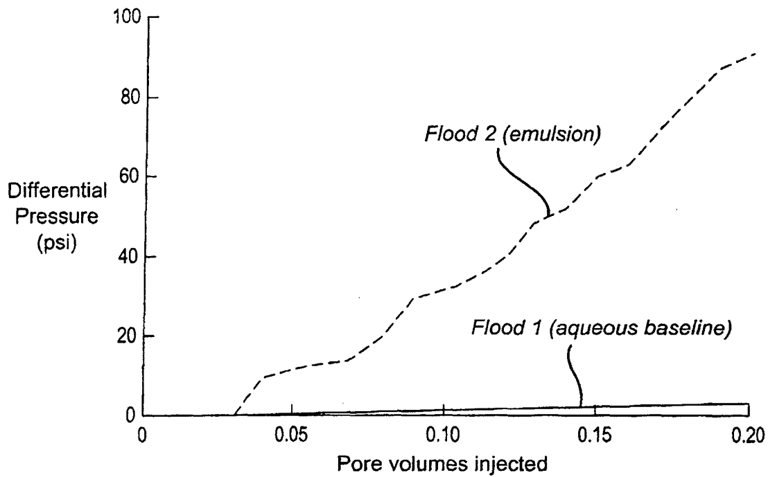
Fig. 1 Differential pressure arising from the scale inhibitor injection stages of corefloods 1 and 2
