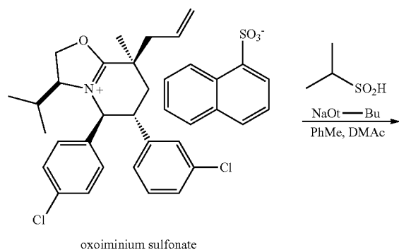
Scheme B
