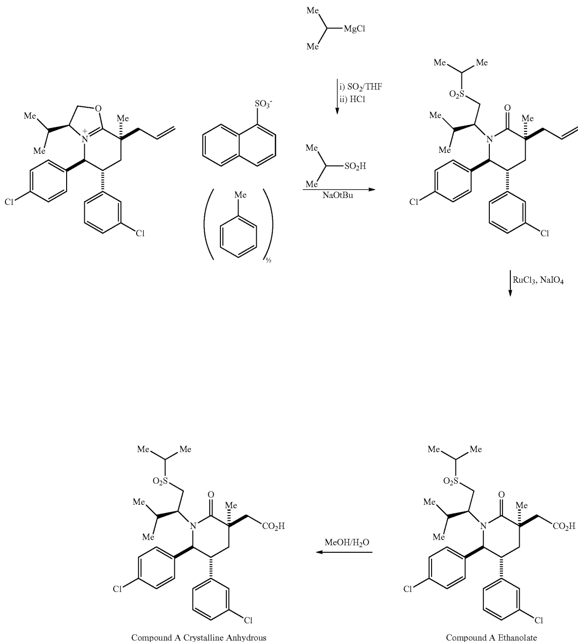
Scheme 1-Procedure 1
