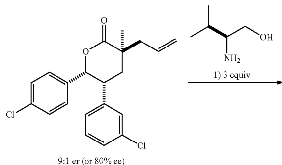
Scheme D
