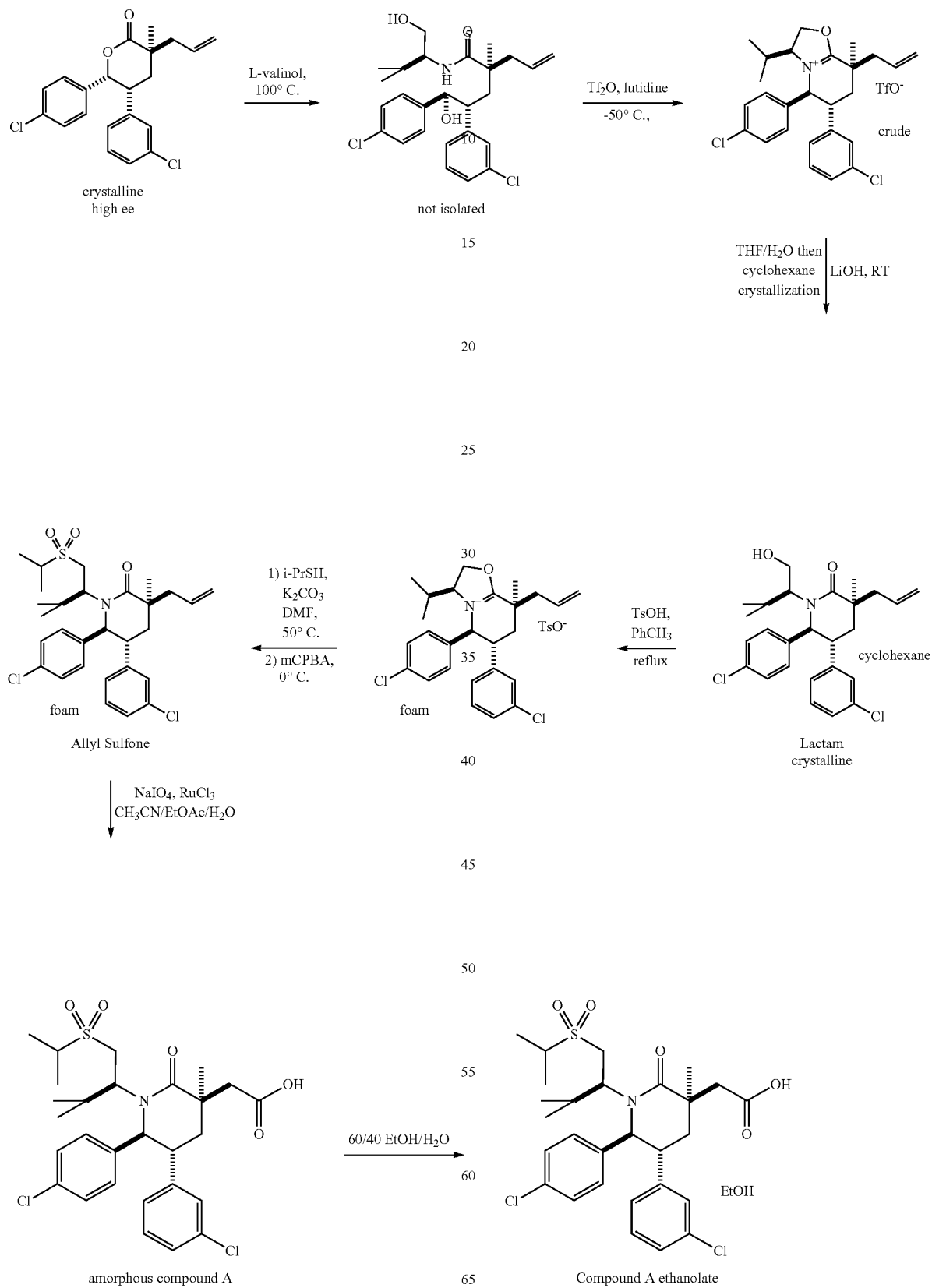
Scheme A
