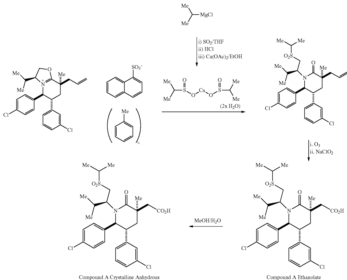
Scheme 2-Procedure 2
