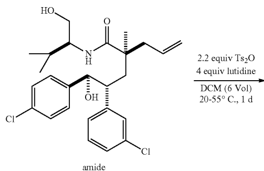
Scheme E
