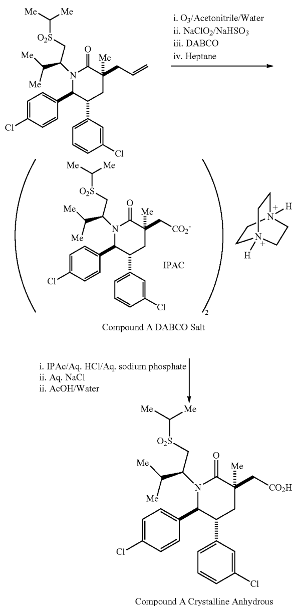
Scheme 3-DABCO Salt Process
