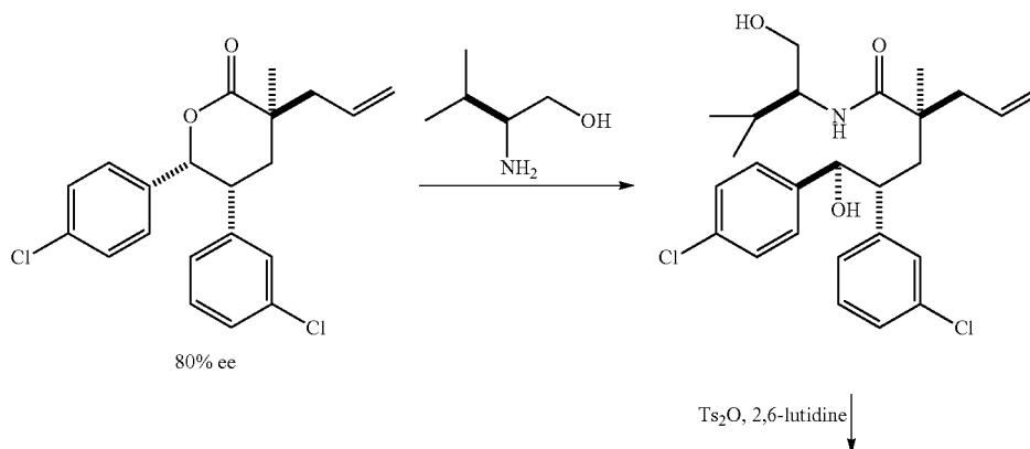
Scheme F
