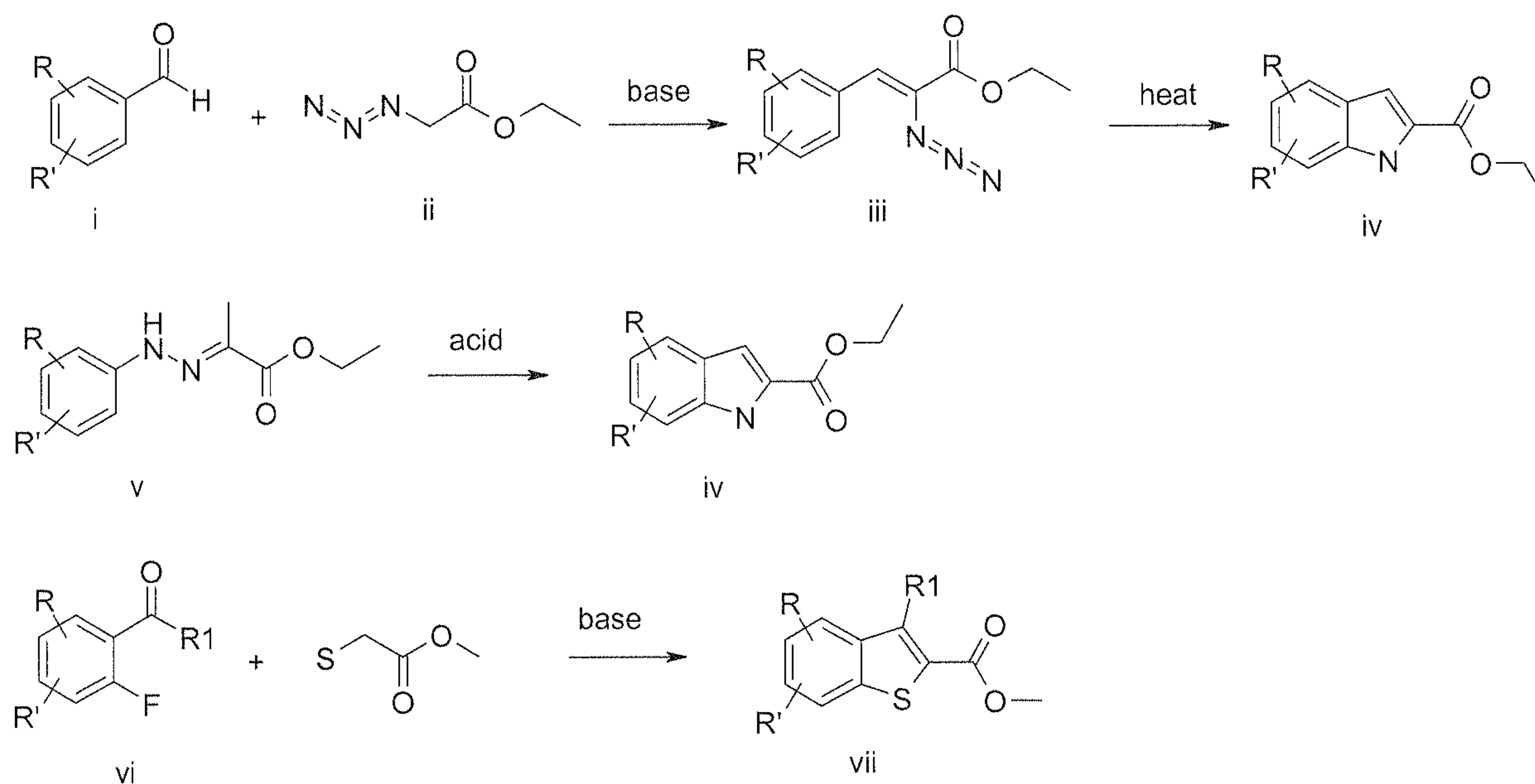
Scheme 1: Preparation of indole and benzothiophene
