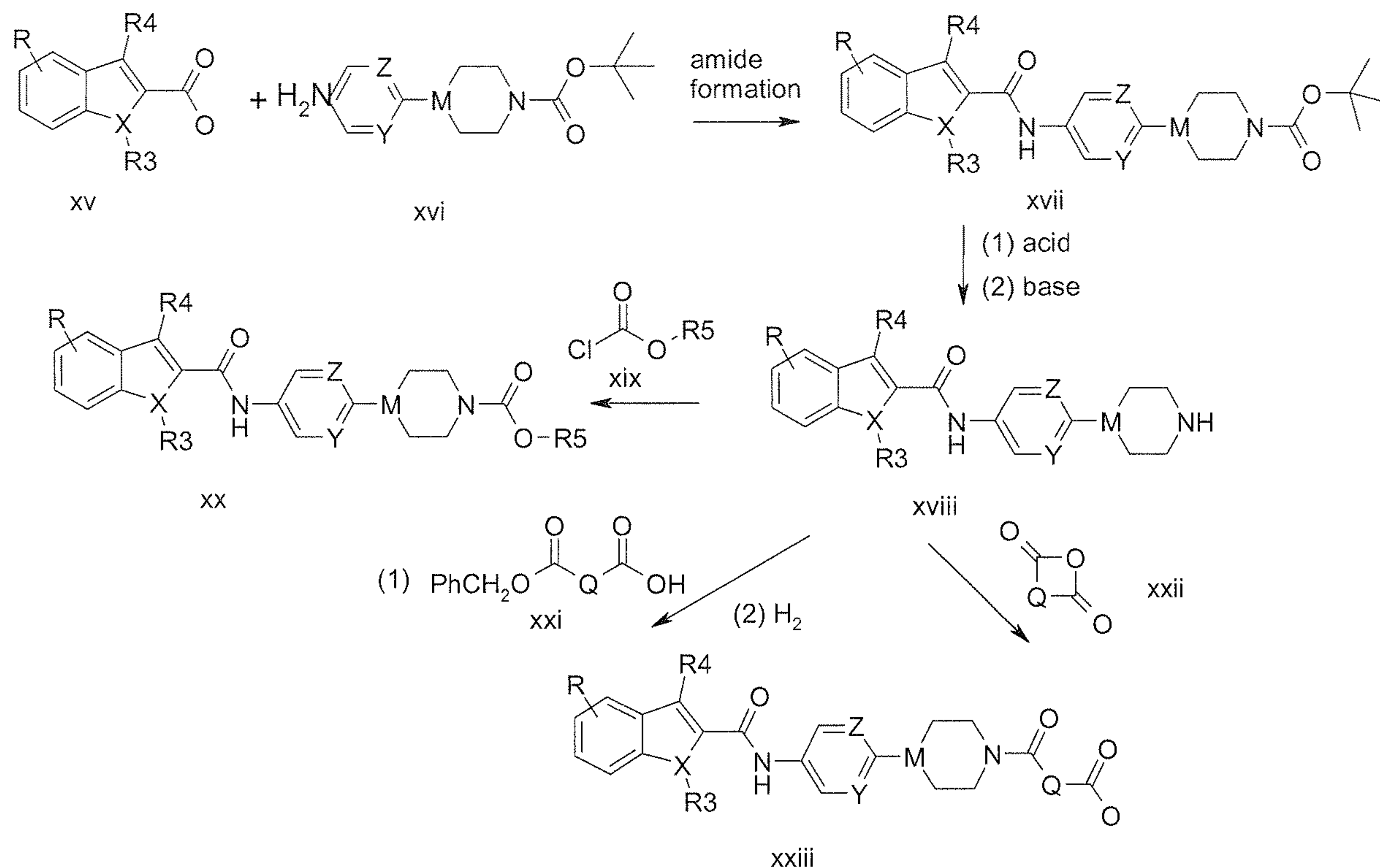
Scheme 3: Preparation of preferred carboxylic acids or carbamates
