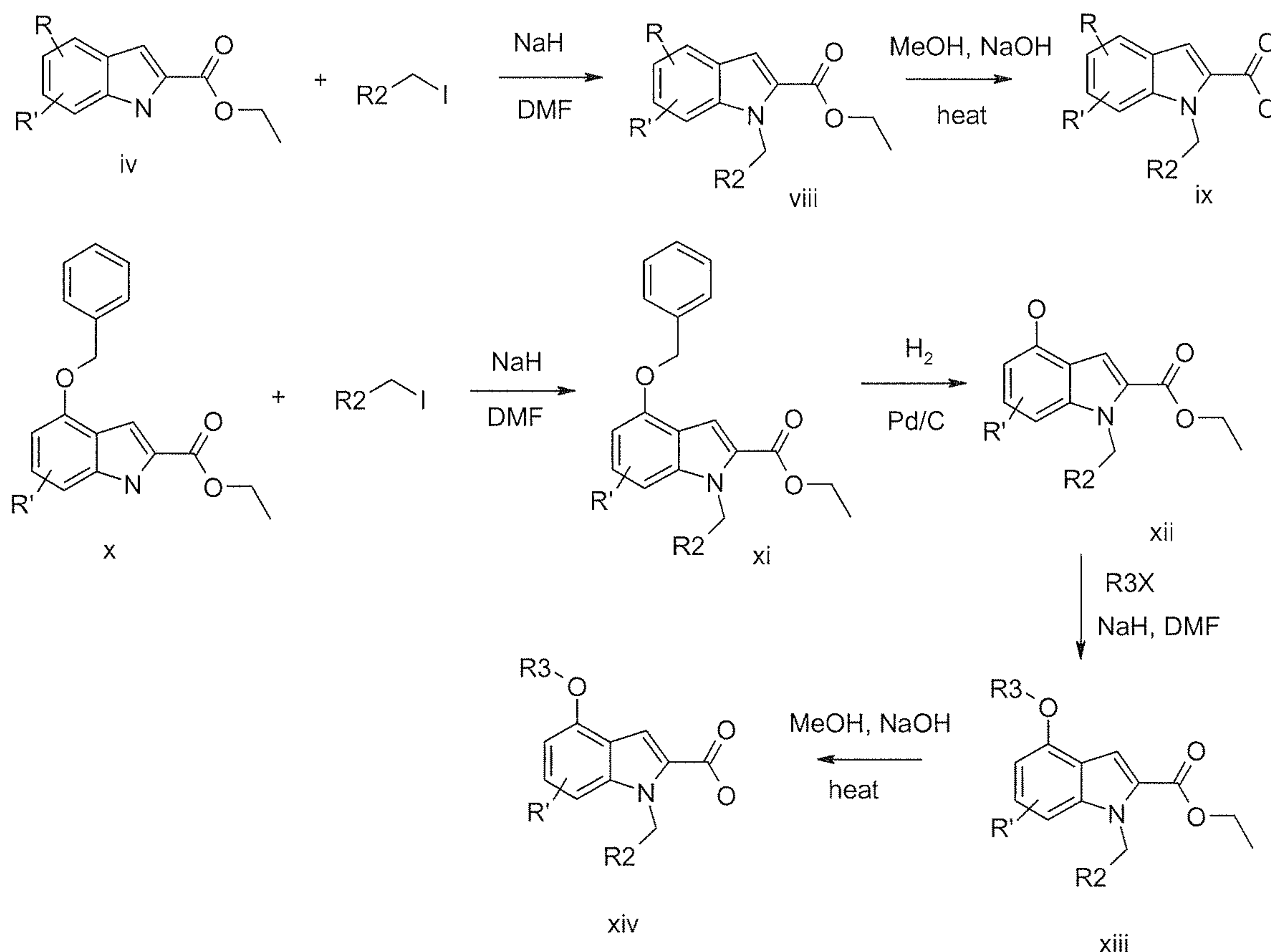
Scheme 2: Preparation of N-alkyl-indole-2-carboxylic acid
