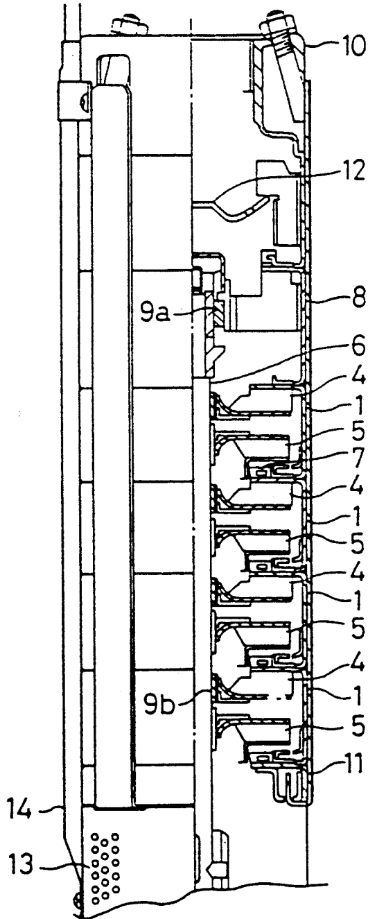
FIG. 7 PRIOR ART
