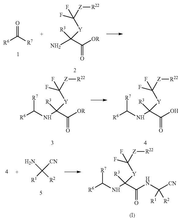
Reaction Scheme 1
