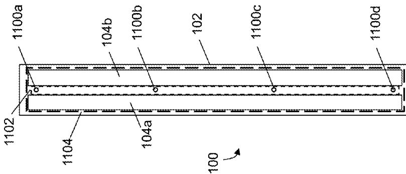
FIG. 11A (Top View)
