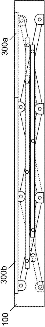
FIG. 10A (Side View)
