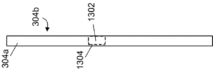
FIG. 13B (Side View)
