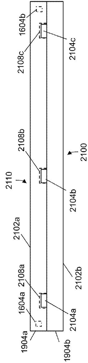
FIG. 21P (Top View)
