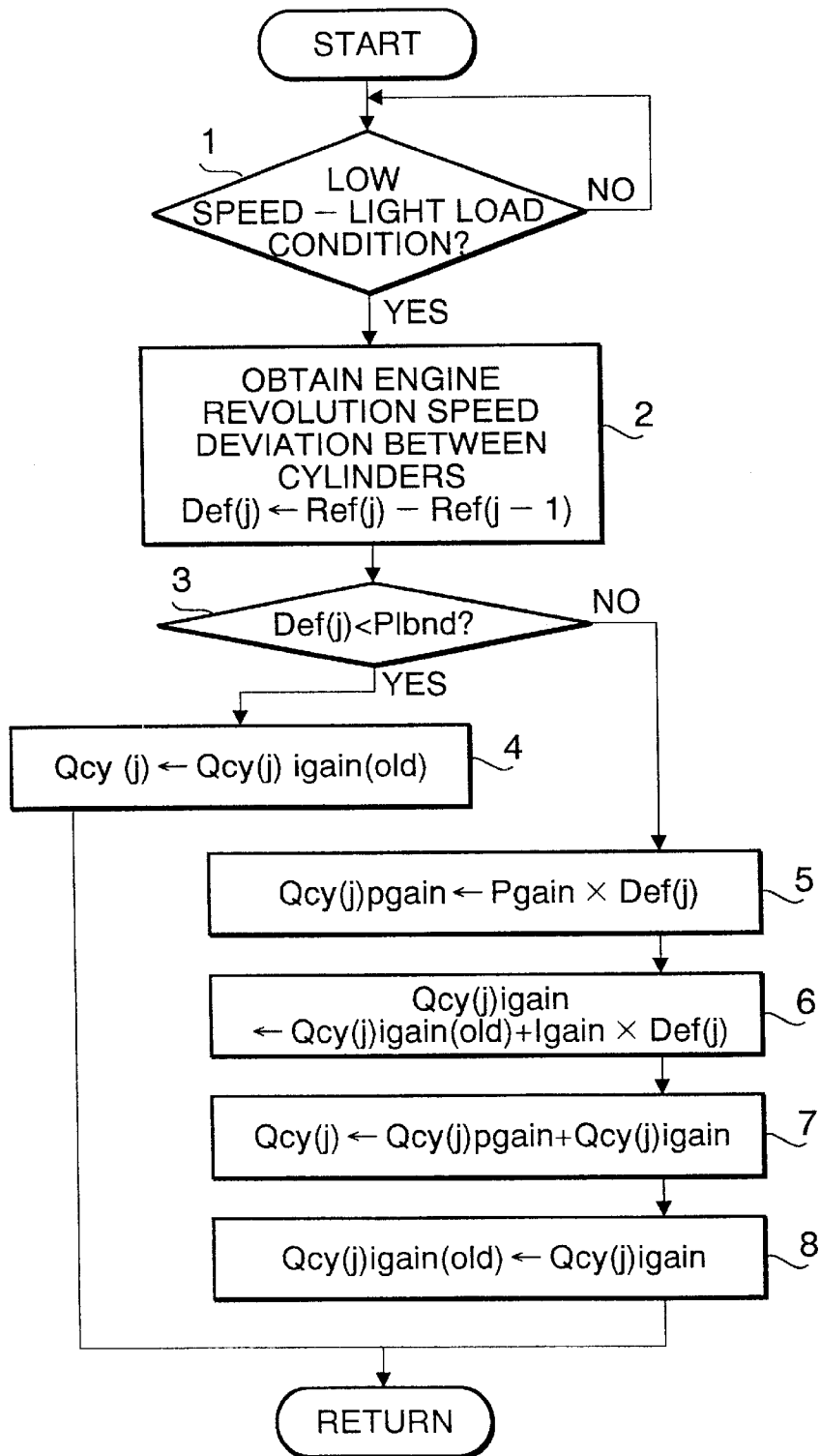
FLOWCHART OF FUEL INJECTION ADJUSTMENT
