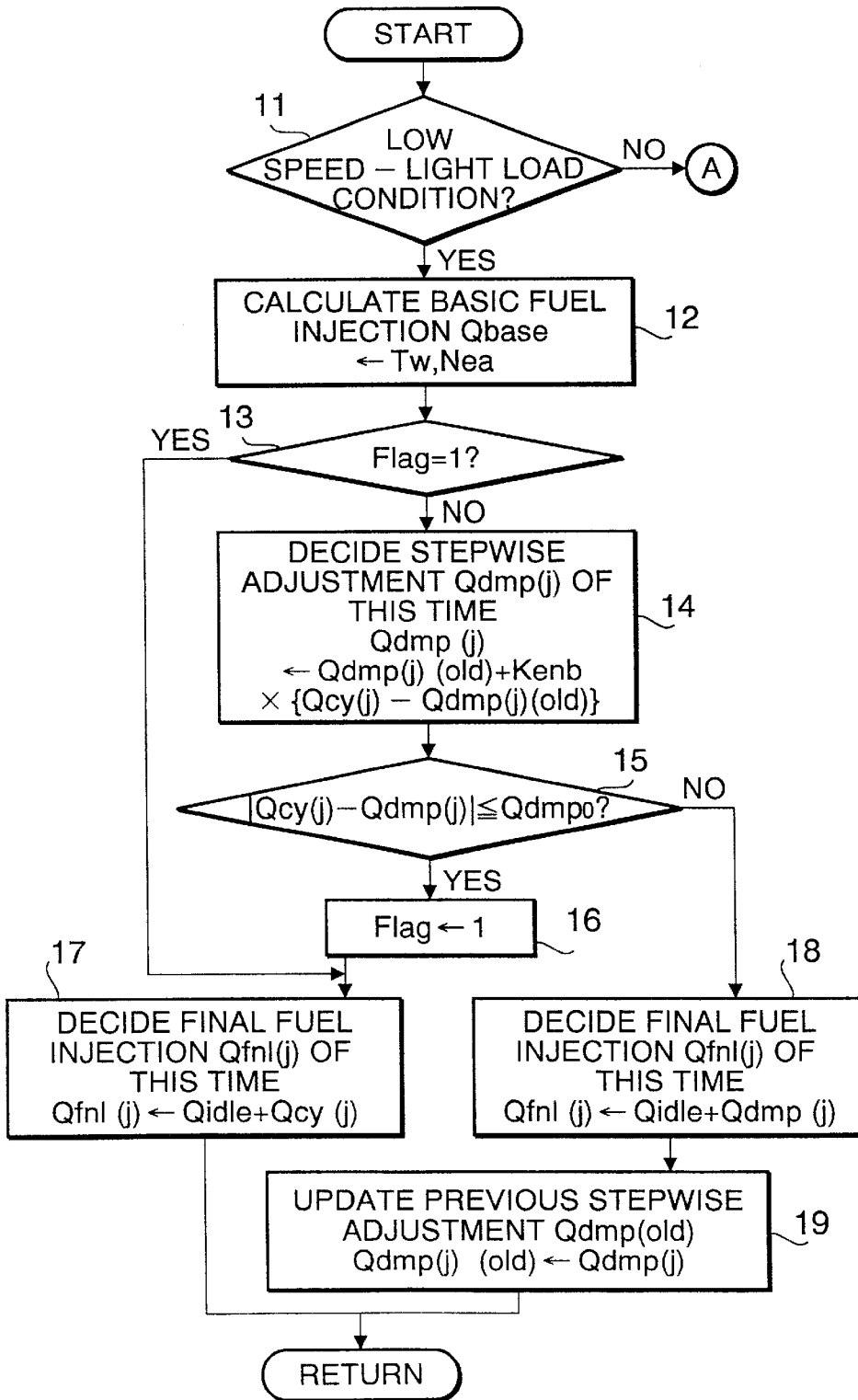
FLOWCHART OF FUEL INJECTION DETERMINATION (1)
