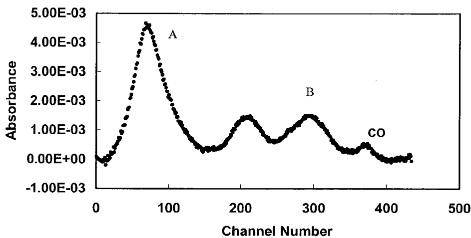
Figure 11 H 2 O and CO spectrum collected on a 500 kW pilot furnace with a 1 ft pathlength. Temperature = 1387 K with a CO concentration of 4.7%.
