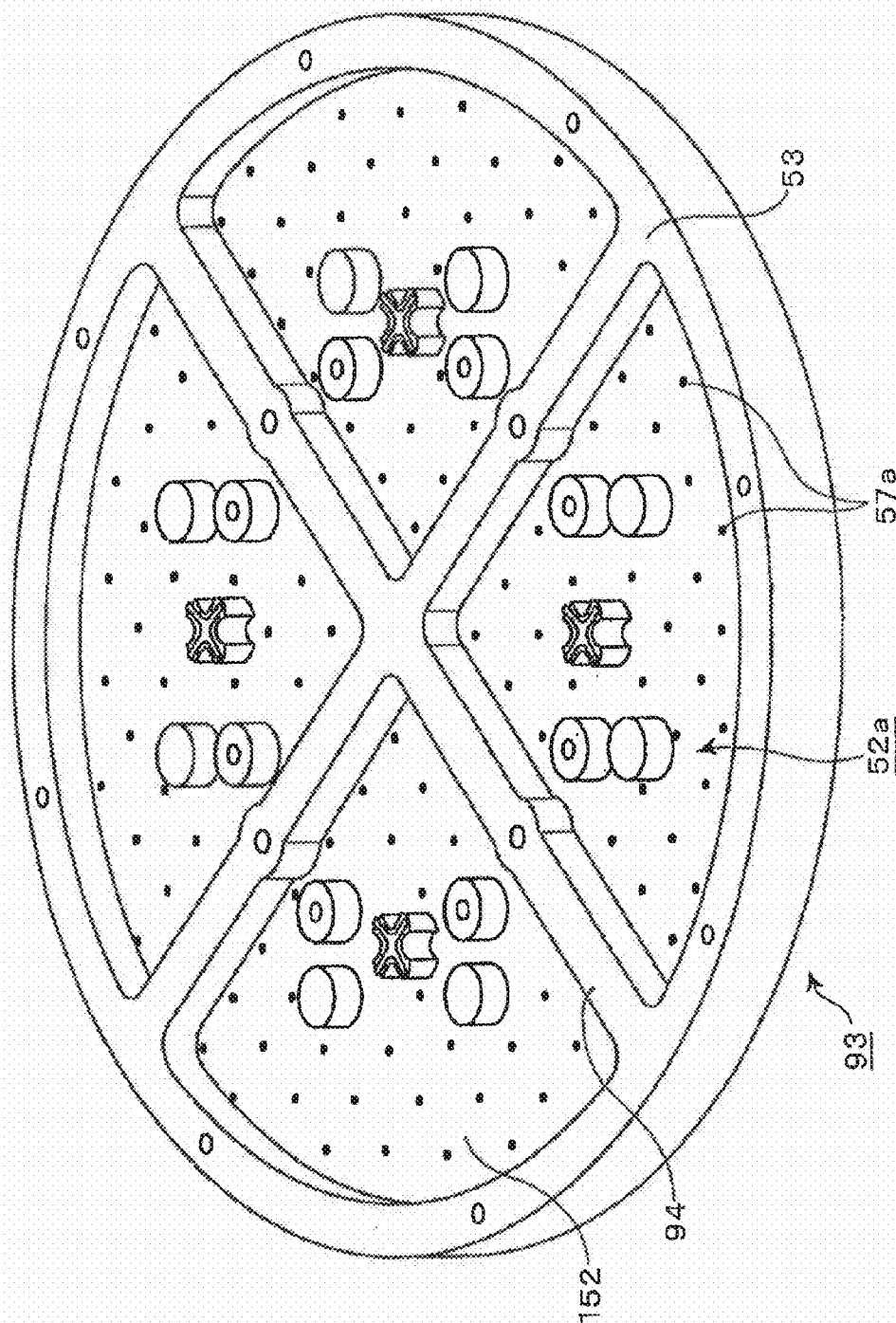
FIG. 13 (PRIOR ART)
