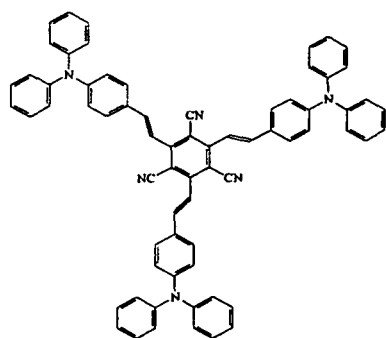
Compound 21
