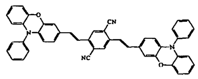
Compound 6
