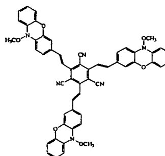
Compound 16
