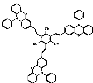
Compound 17
