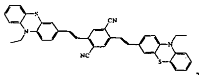
Compound 7
