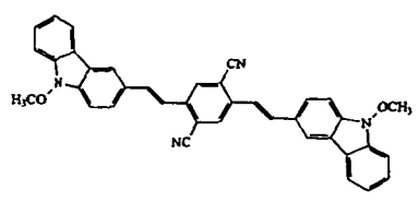
Compound 2
