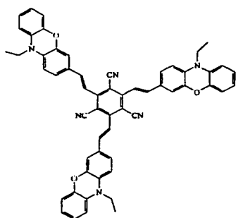
Compound 15
