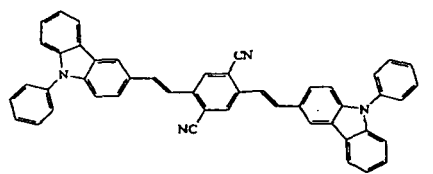
Compound 3
