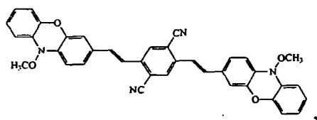
Compound 5
