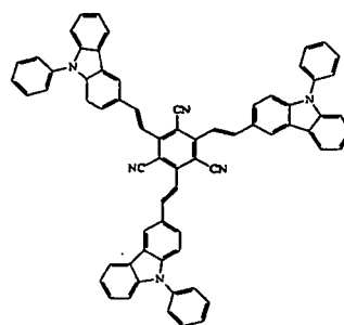
Compound 14
