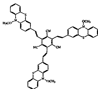
Compound 19
