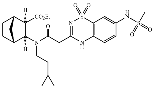
b) (1S,2R,3S,4R)-3-{(2-Cyclopropyl-ethyl)-[2-(7-methanesulfonylamino-1,1-dioxo-1,4-dihydro-1 \lambda^6 -benzo[1,2,4]thiadiazin-3-yl)-acetyl]-amino}-bicyclo[2.2.1]heptane-2-carboxylic acid ethyl ester
