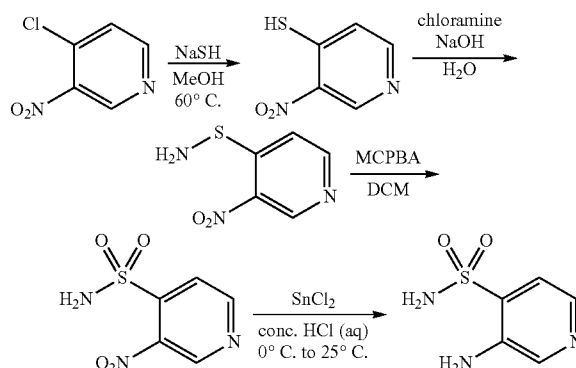
Scheme 19
