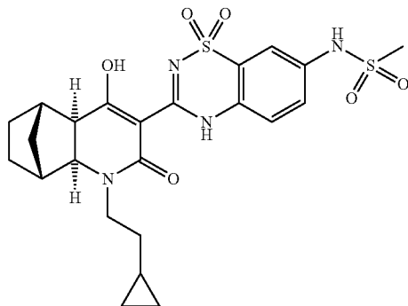
a) (1S,2R,3S,4R)-3-(2-Cyclopropyl-ethylamino)-bicyclo[2.2.1]heptane-2-carboxylic acid ethyl ester
