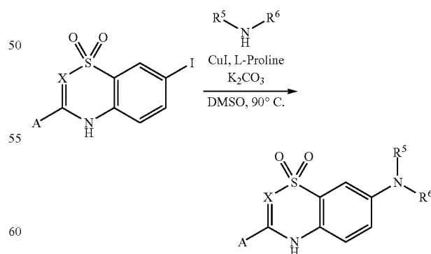
Scheme 28
