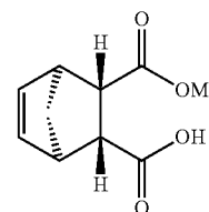
a) (1R,2R,3S,4S)-3-(Methoxycarbonyl)bicyclo[2.2.1]hept-5-ene-2-carboxylic acid
