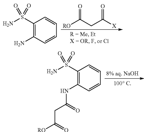
Scheme 18
