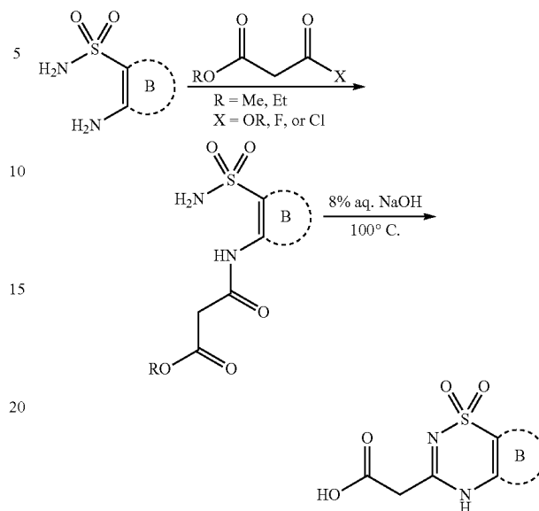
Scheme 23
