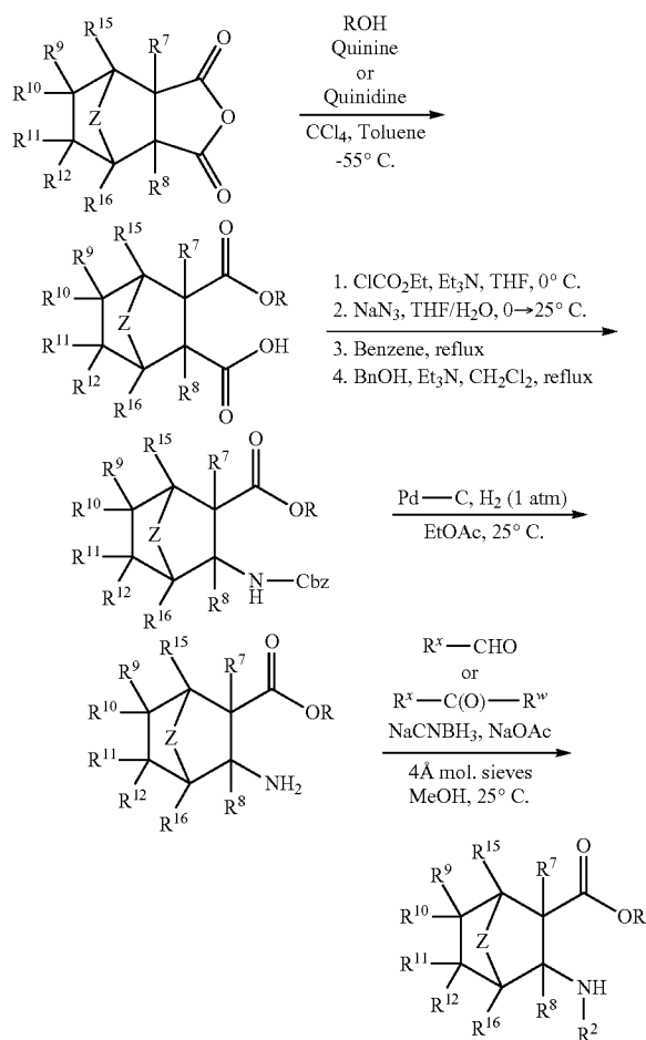
Scheme 3
