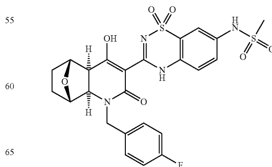
d) N-{3-[(1S,2R,7S,8R)-3-(4-Fluoro-benzyl)-6-hydroxy-4-oxo-11-oxa-3-aza-tricyclo[6.2.1.0 2,7 ]undec-5-en-5-yl]-1,1-dioxo-1,4-dihydro-1λ 6 -benzo[1,2,4]thiadiazin-7-yl]-methanesulfonamide
