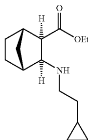
a) (1S,2R,3S,4R)-3-(2-Cyclopropyl-ethylamino)-bicyclo[2.2.1]heptane-2-carboxylic acid ethyl ester
