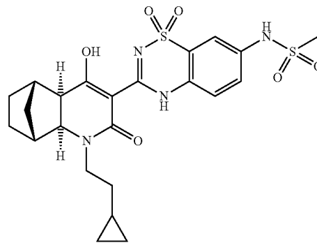
c) N-{3-[(1R,2S,7R,8S)-3-(2-Cyclopropyl-ethyl)-6-hydroxy-4-oxo-3-aza-tricyclo[6.2.1.0 2,7 ]undec-5-en-5-yl]-1,1-dioxo-1,4-dihydro-1 \lambda^6 -benzo[1,2,4]thiadiazin-7-yl]-methanesulfonamide
