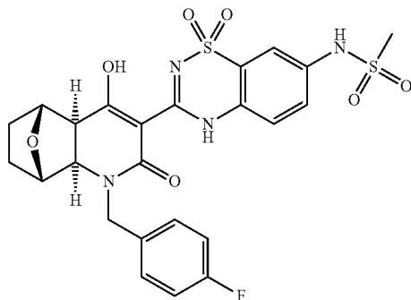
a) (rac-di-exo)-Methyl 3-amino-7-oxabicyclo[2.2.1]heptane-2-carboxylate
