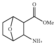
a) (rac-di-exo)-Methyl 3-amino-7-oxabicyclo[2.2.1]heptane-2-carboxylate
