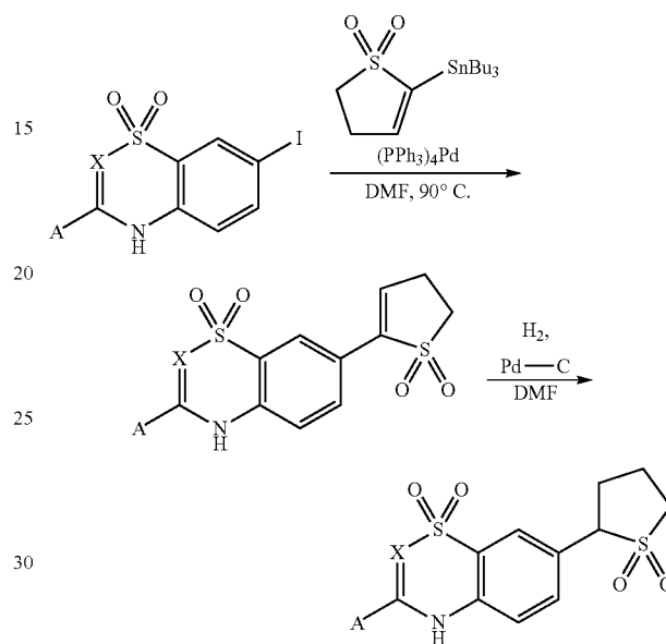
Scheme 27
