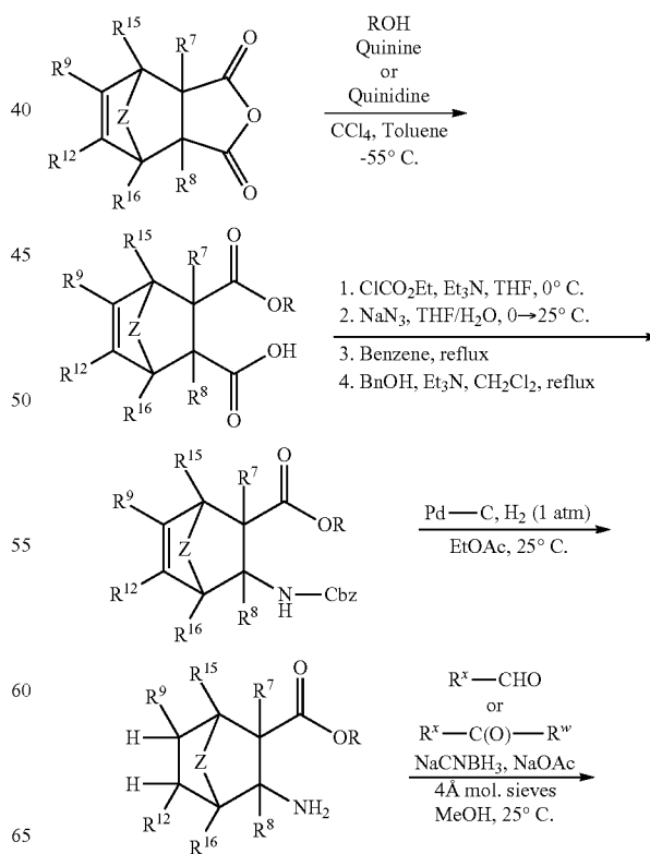
Scheme 4
