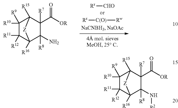
Scheme 9
