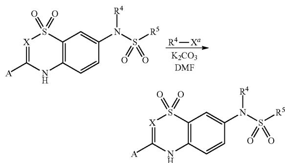
Scheme 26
