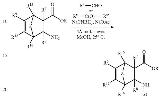
Scheme 11
