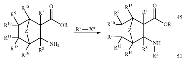
Scheme 10
