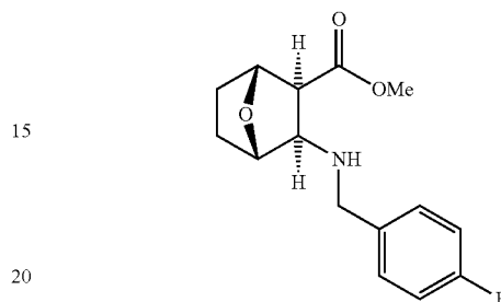
c) Methyl (1R,2S,3R,4S)-3-[(4-fluorobenzyl)amino]-7-oxabicyclo[2.2.1]heptane-2-carboxylate
