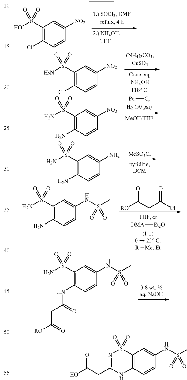
Scheme 14
