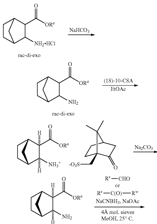
Scheme 7
