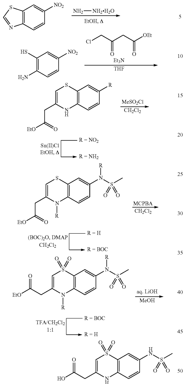
Scheme 13
