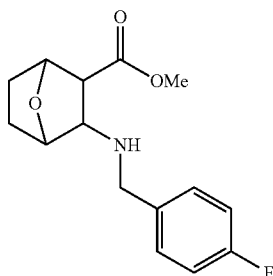
b) (rac-di-exo)-Methyl 3-[(4-fluorobenzyl)amino]-7-oxabicyclo[2.2.1]heptane-2-carboxylate
