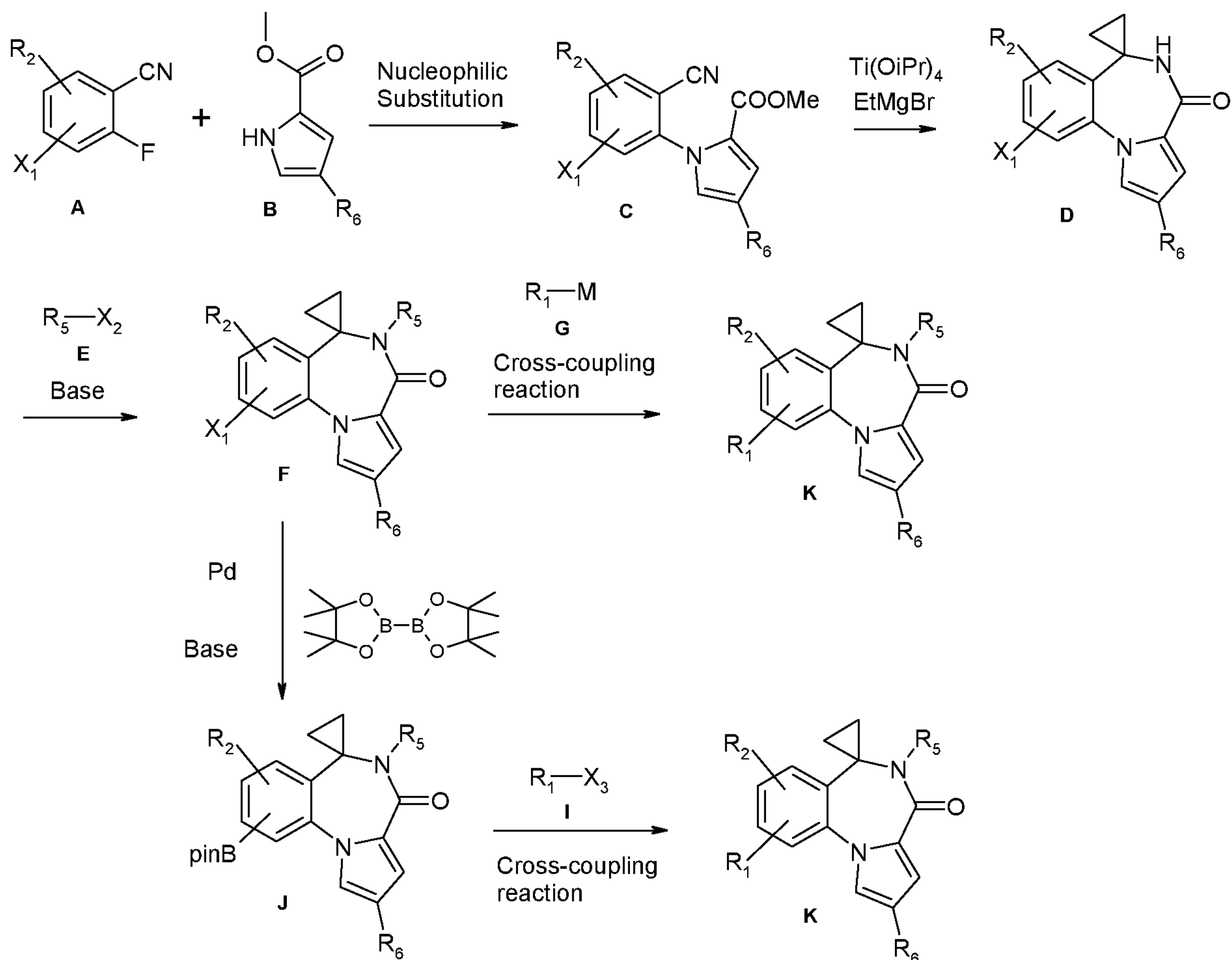
Scheme 1:
