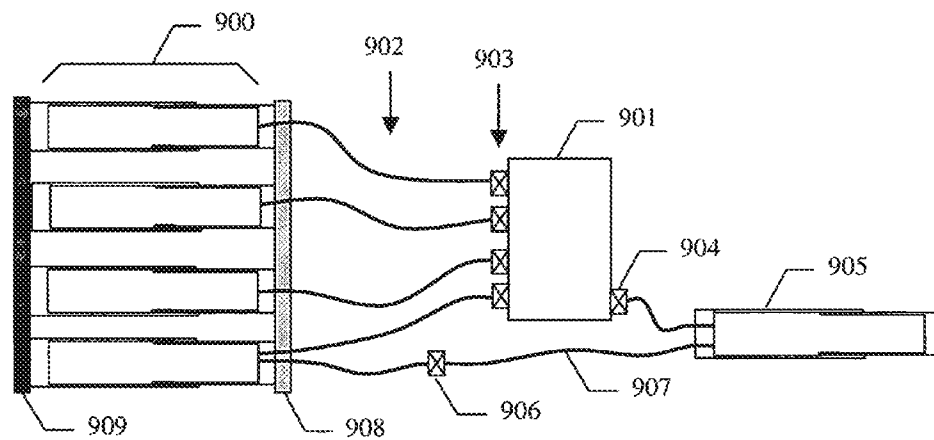
Variable-Spring-Rate Multiple-Pneumatic-Chamber and Energy Transfer System.
