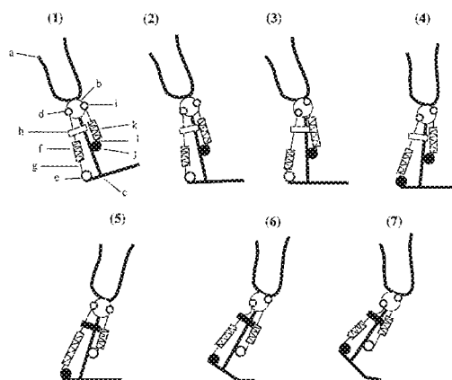
External, Bi-articular Transfemoral Prosthesis, Robotic Limb, or Orthotic Brace in Heel- Strike to Toe-Off Walking Sequence
