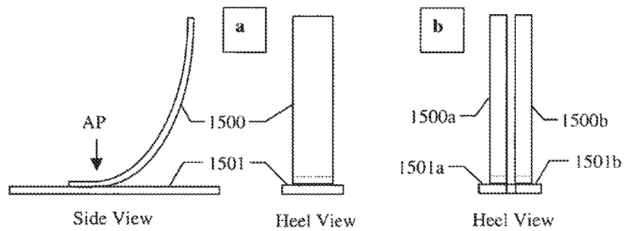
Prior-Art Prosthetic Ankle-Foot
