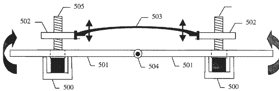
Variable Spring-Rate Joint
