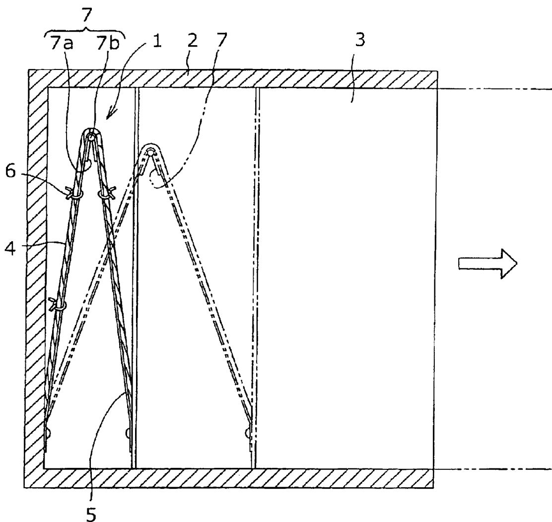
Fig.12 Prior Art
