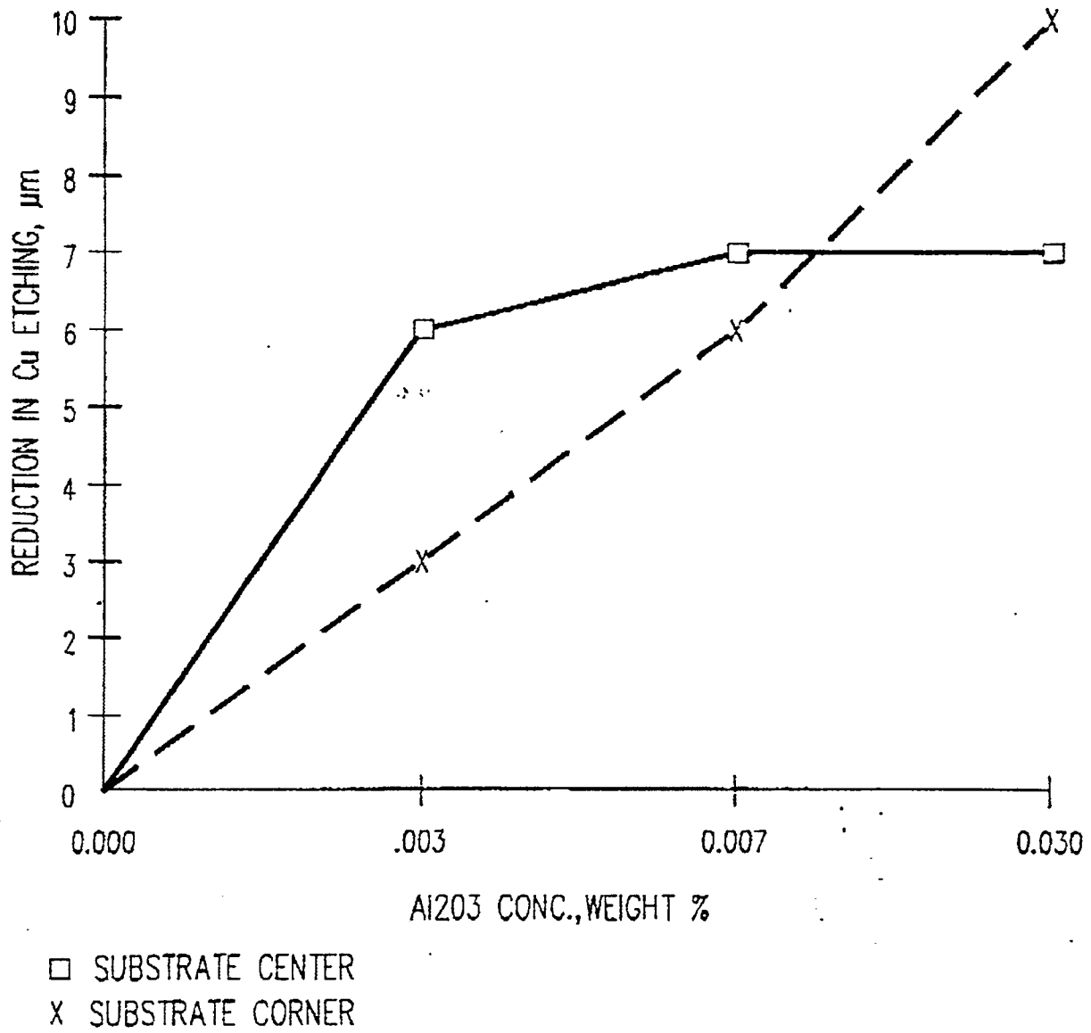
Cu ETCH REDUCTION WITH Al 2 O 3 ADDITION
