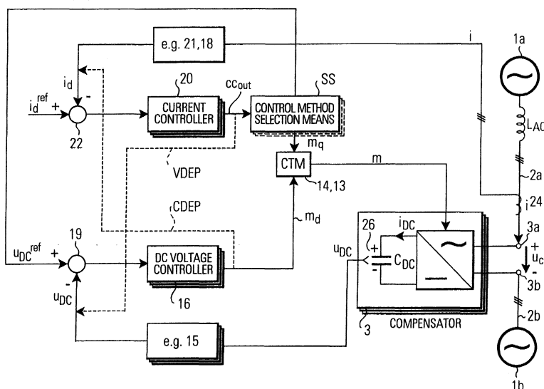
FIG.18a PRINCIPLE OF THE INVENTION
