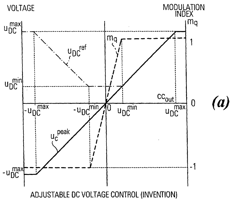
FIG.22 STATIC CHARACTERISTICS
