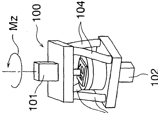
FIG. 6D M z APPLIED
