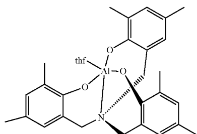
Amino-triphenolate complex
