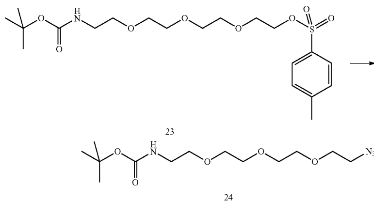
Compound 24 tert-Butyl (2-{2-[2-(2-azidoethoxy)ethoxy] ethoxy}ethyl)carbamate
