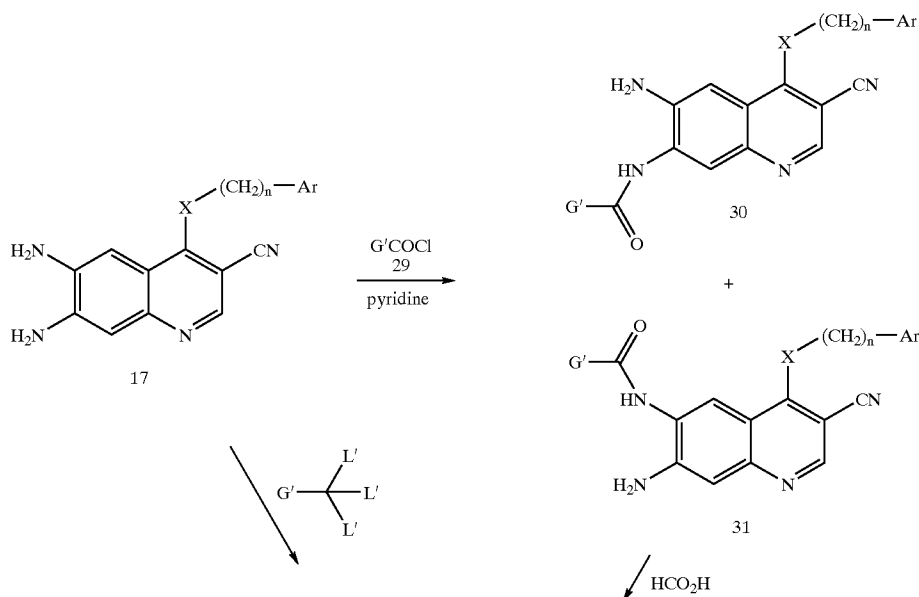
Flowsheet 8
