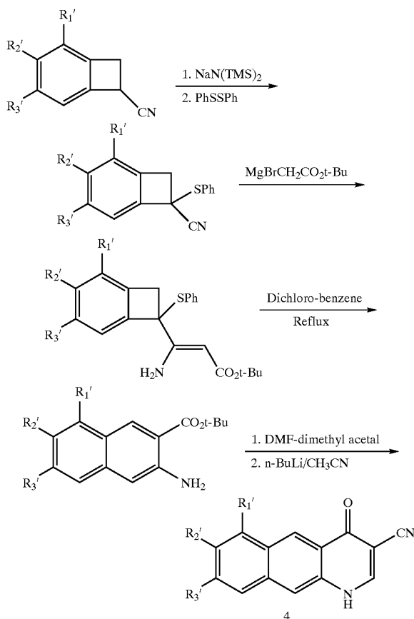
Flowsheet 1'''
