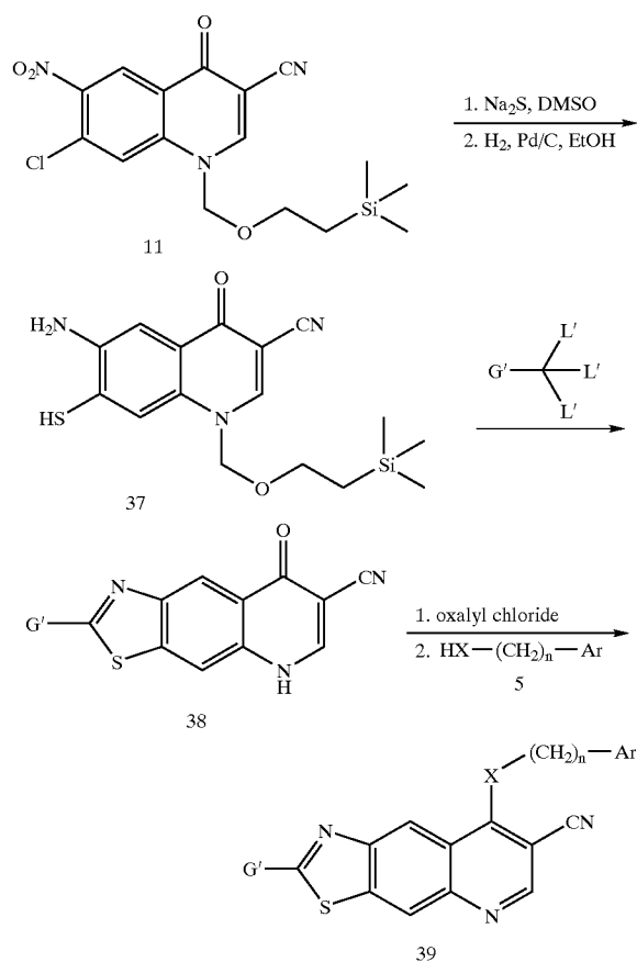
Flowsheet 10
