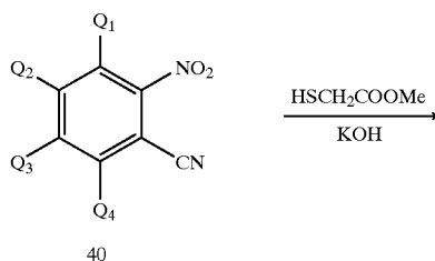
Flowsheet 11
