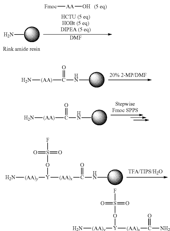
Scheme 2. Overview of \text{Y}(\text{OSO}_2\text{F}) -containing peptide synthesis
