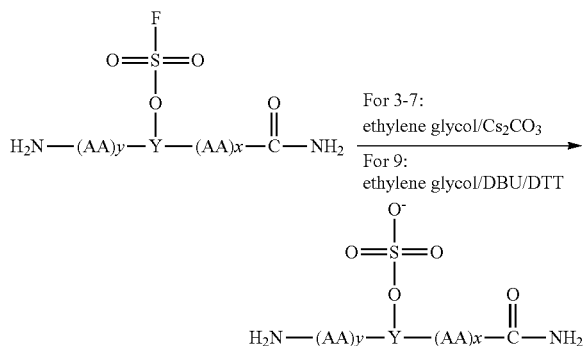
Scheme 3. Overview of arylfluorosulfate hydrolysis to afford sY peptides
