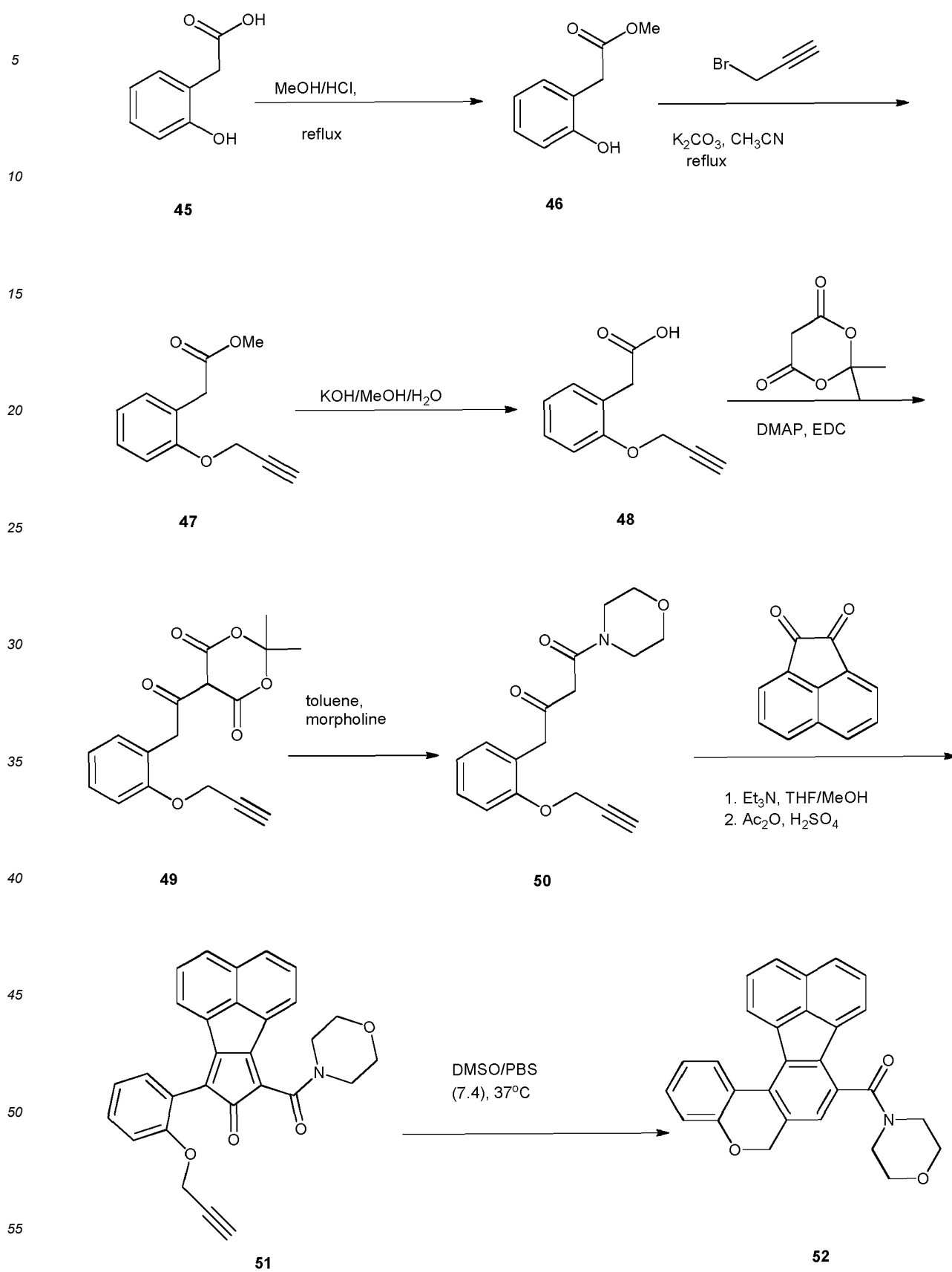
Scheme 15.
