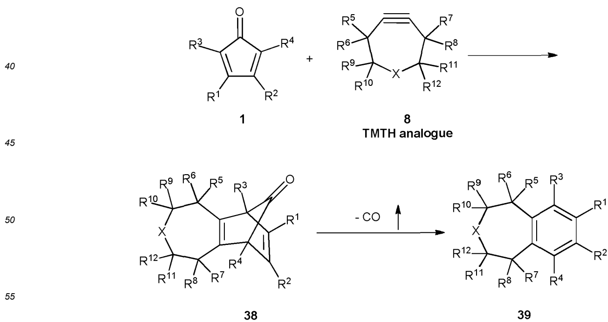
Scheme 8.
