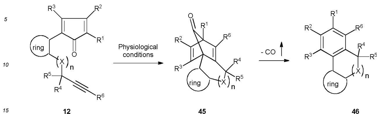
Scheme 11.
