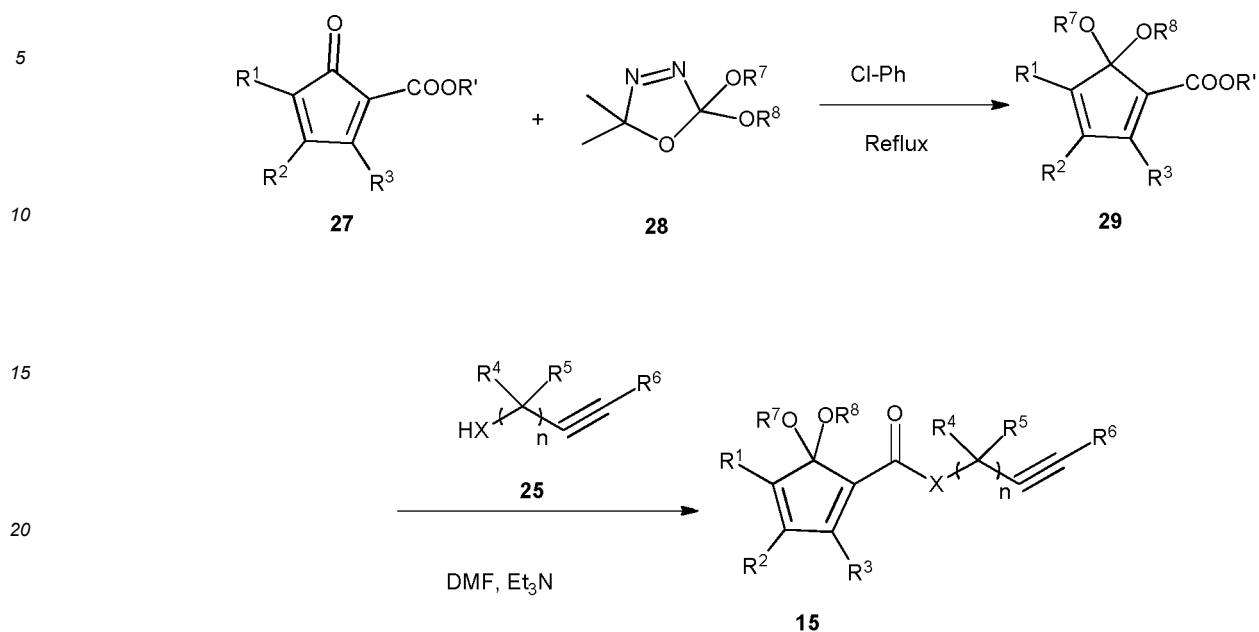
Scheme 3.
