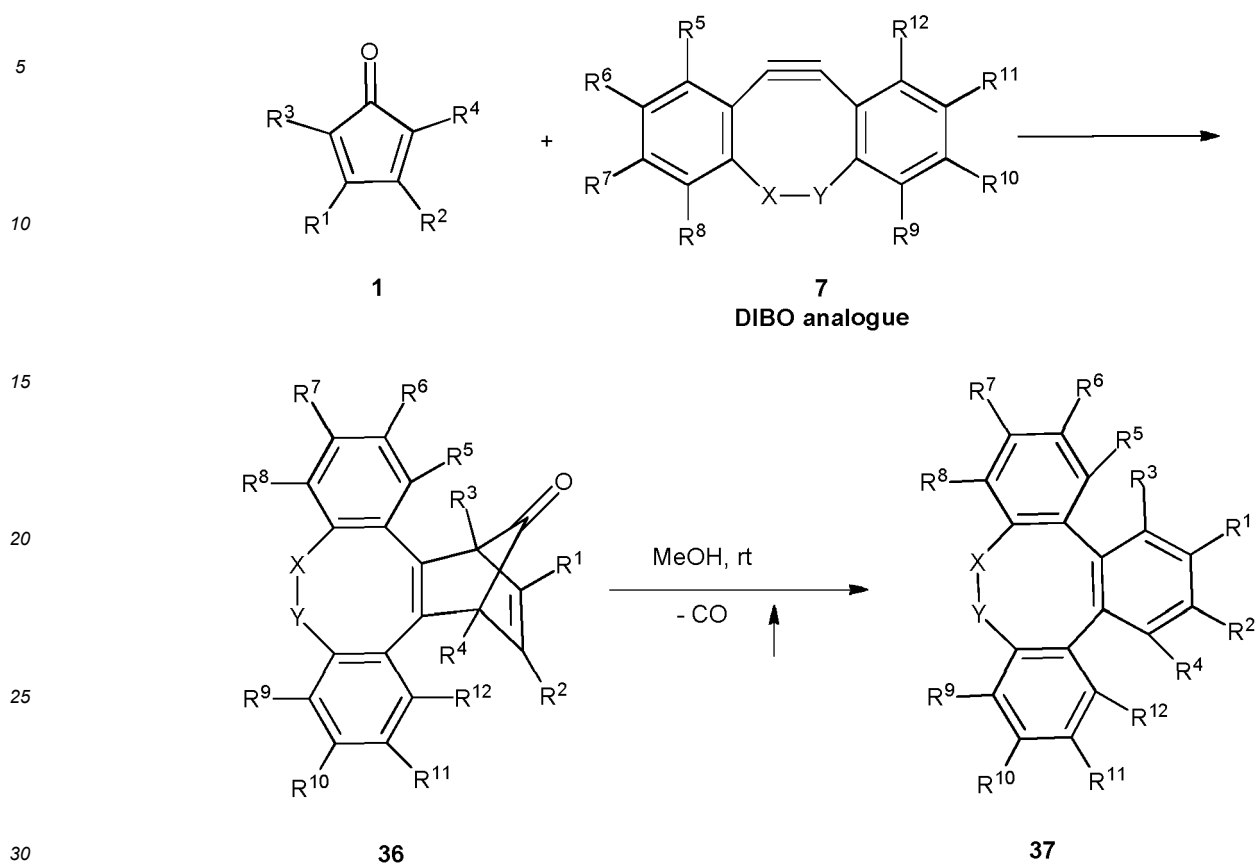
Scheme 7.
