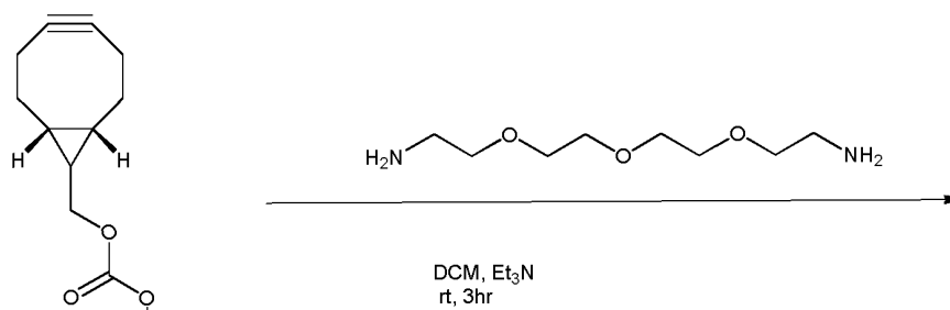
Scheme 17—cont'd.
