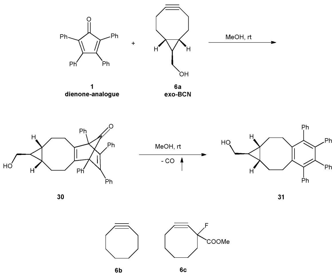
Scheme 12.
