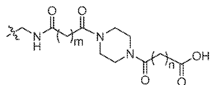
[00124] Scheme 5
