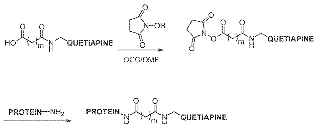
[00128] Scheme 7
