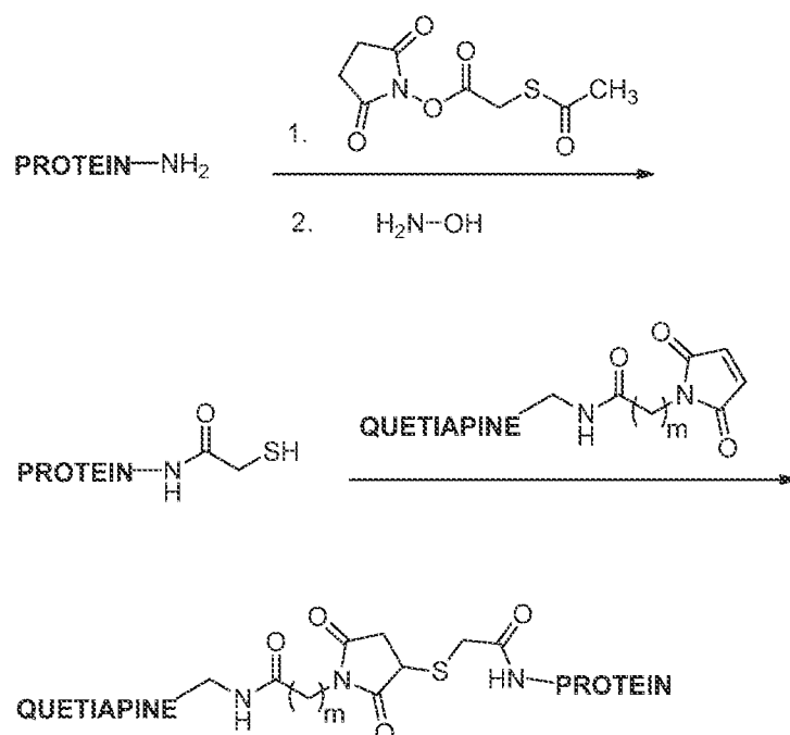
[00126] Scheme 6
