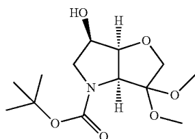
(3aS, 6aS)-6R-hydroxy-3,3-dimethoxy-hexahydro-furo[3,2-b]pyrrole-4-carboxylic Acid Tert-Butyl Ester (1d)
