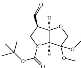
6-Formyl-3,3-dimethoxy-hexahydro-furo[3,2-b]pyrrole-4-carboxylic Acid Tert-Butyl Ester (1h)
