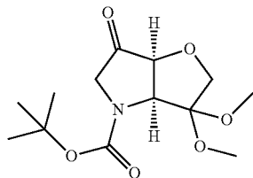
3,3-Dimethoxy-6-oxo-hexahydro-furo[3,2-b]pyrrole-4-carboxylic Acid Tert-Butyl Ester (1e)
