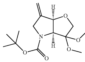
3,3-Dimethoxy-6-methylene-hexahydro-furo[3,2-b]pyrrole-4-carboxylic Acid Tert-Butyl Ester (1f)
