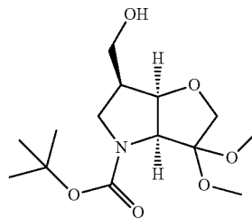
6-Hydroxymethyl-3,3-dimethoxy-hexahydro-furo[3,2-b]pyrrole-4-carboxylic Acid Tert-Butyl Ester (1g)
