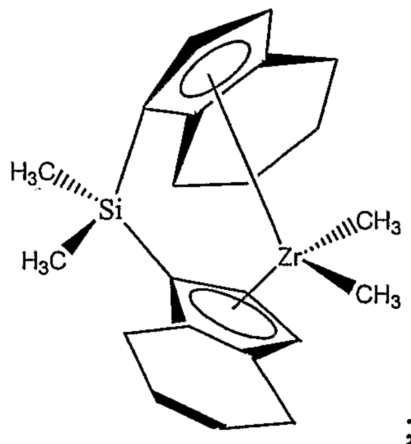
dimethylsilylbis(2-methyl-1-indenyl)zirconium dibenzyl,
