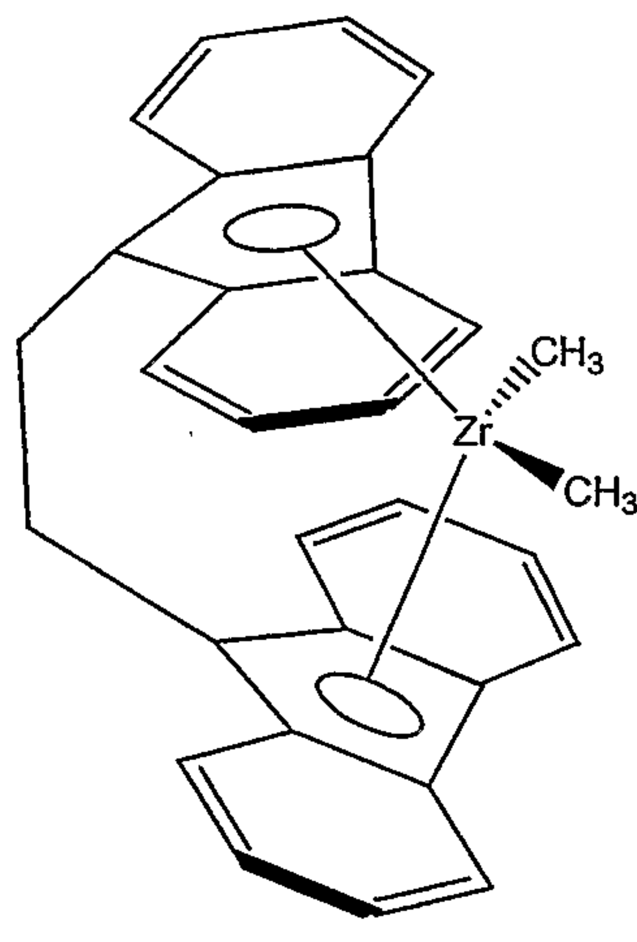
(indenyl)trisbenzyl titanium(IV),
