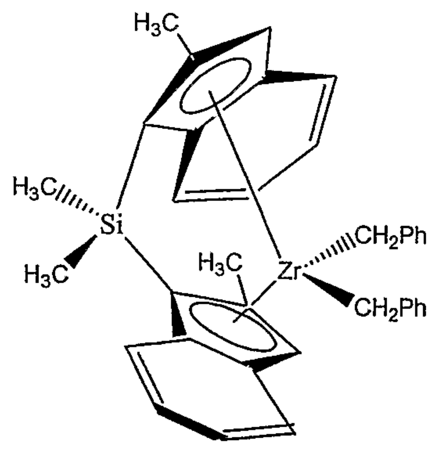
1,2-ethanediylbis(9-fluorenyl)zirconium dimethyl,
