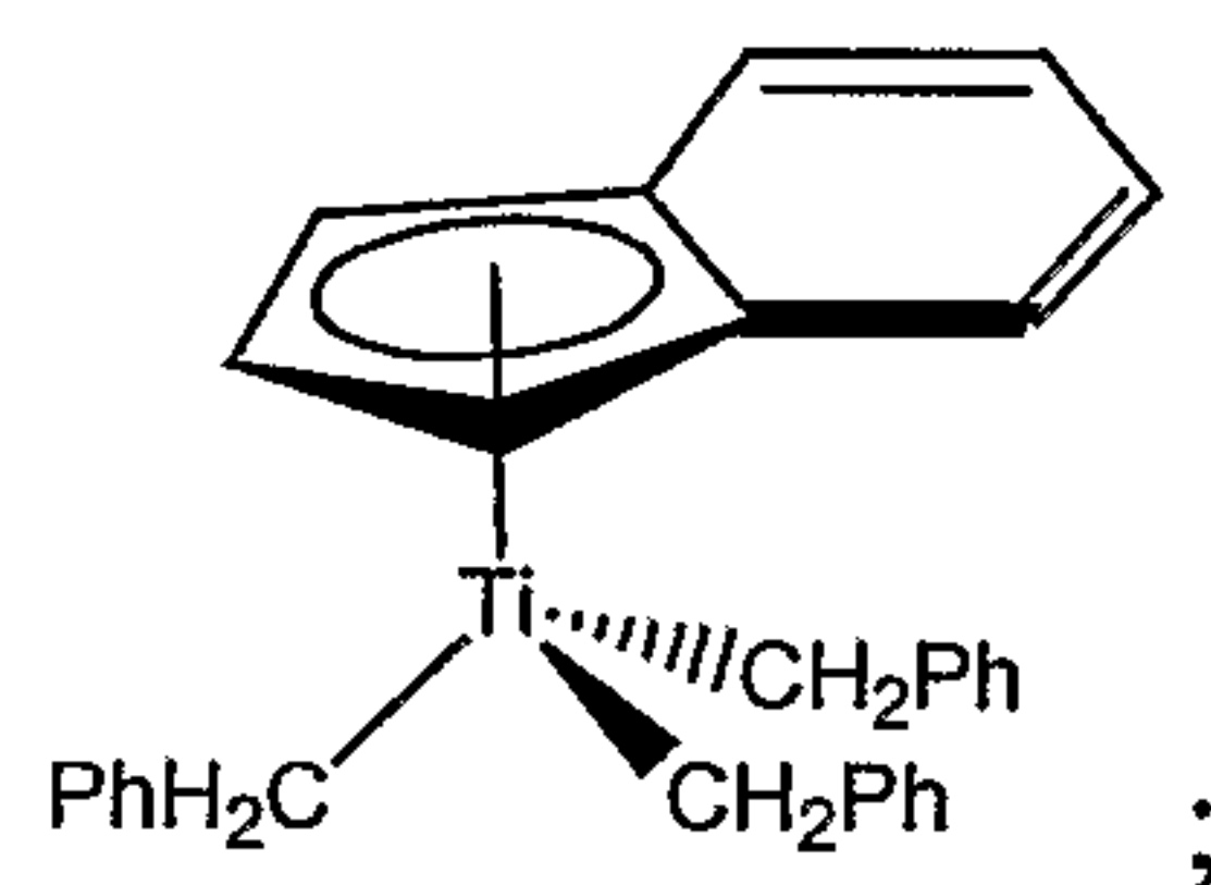
(isopropylamidodimethylsilyl)cyclopentadienyltitanium dibenzyl,
