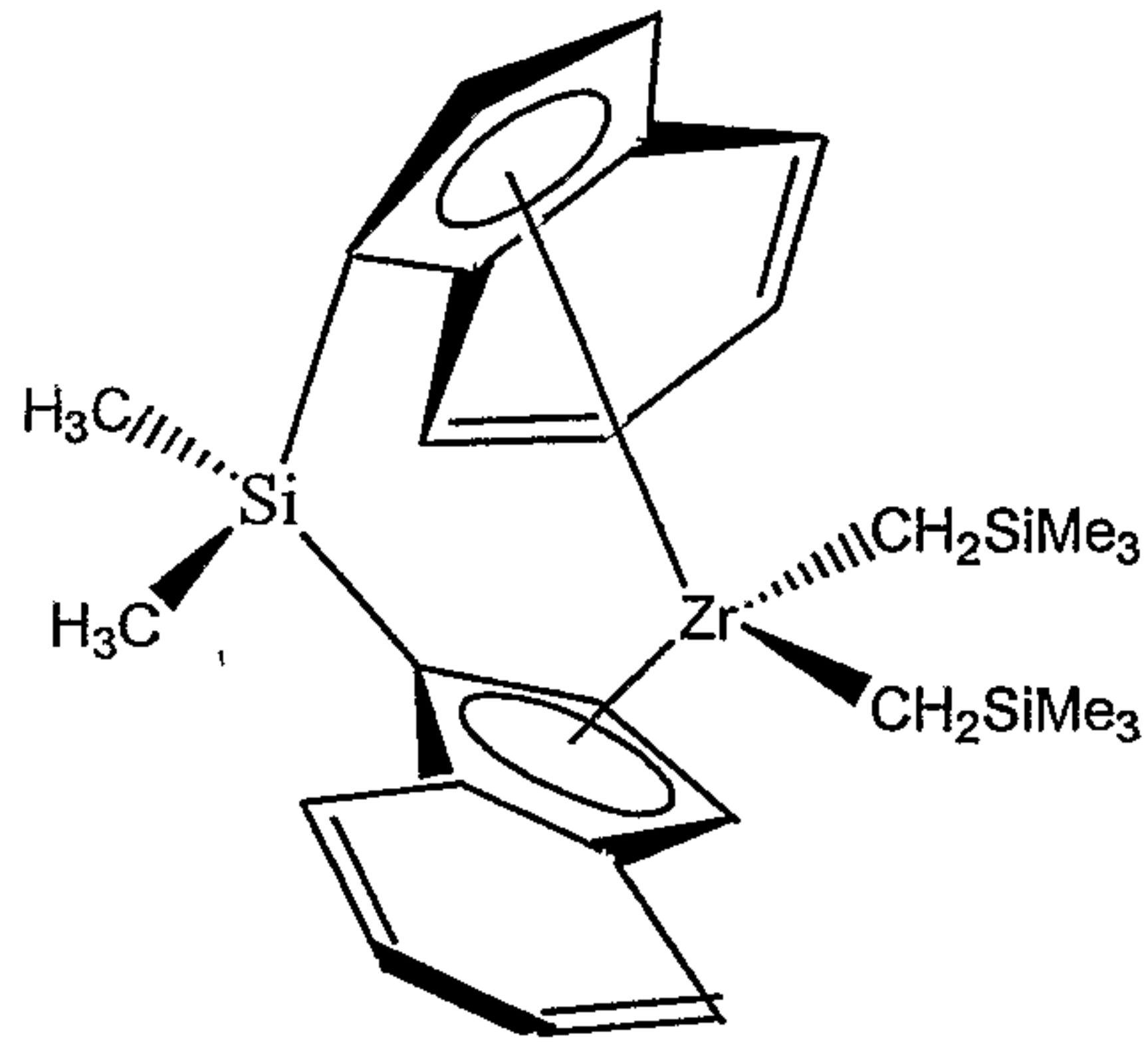
octyl(phenyl)silylbis(1-indenyl)hafnium dimethyl,
