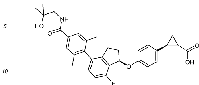
Example 54 in WO 2013/178575
