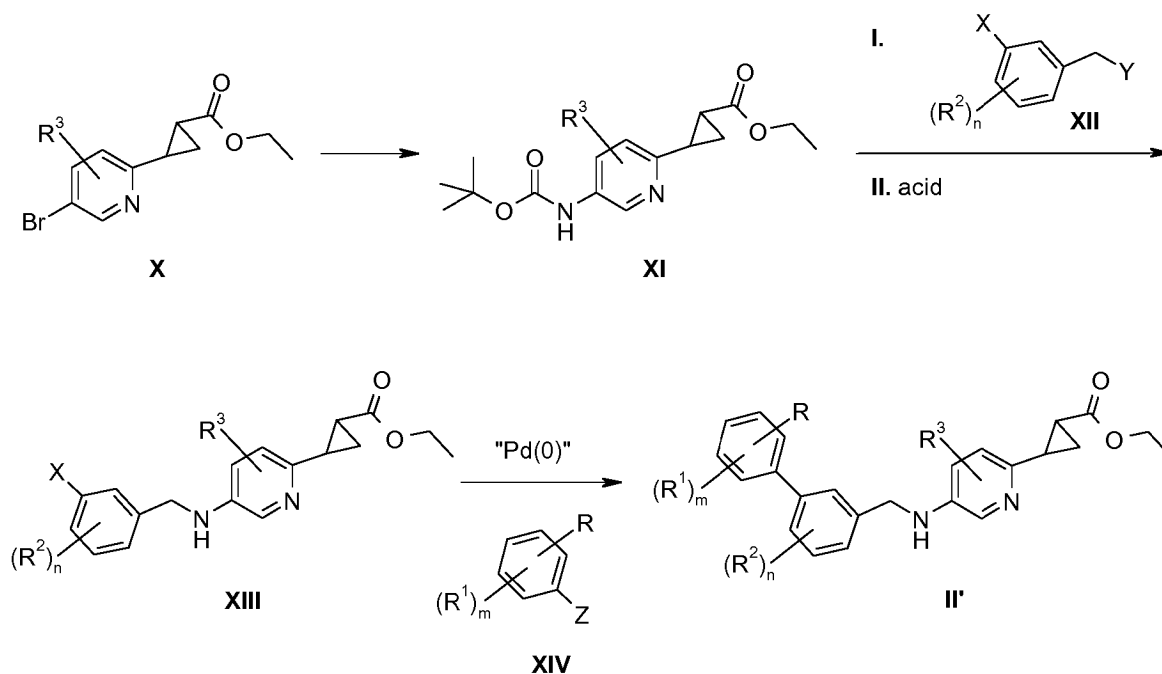
Scheme 4: Alternative Approach for the synthesis of intermediate II
