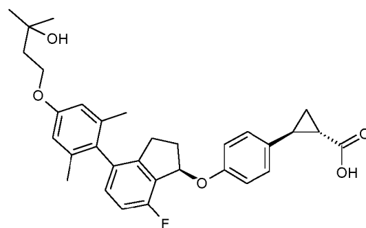
Example 45 in WO 2013/178575
