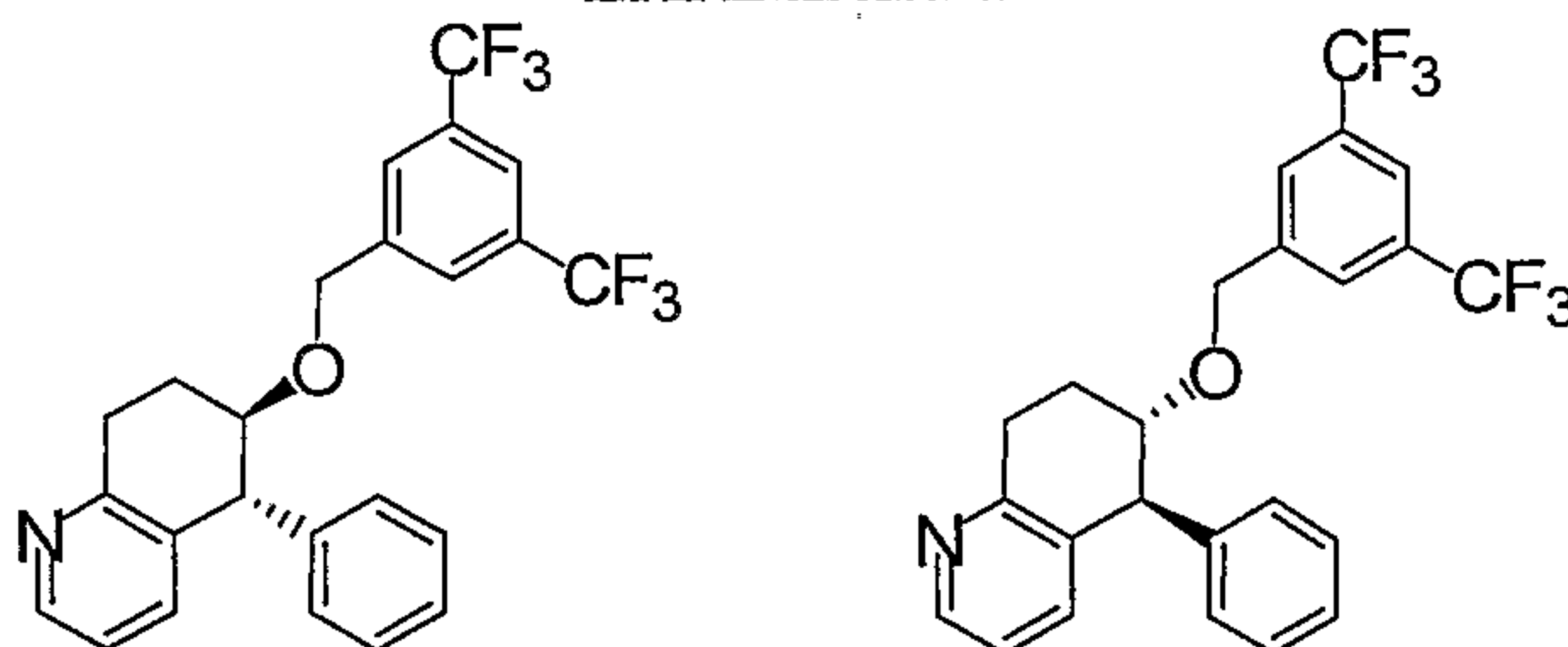
Racemic-(5,6-trans)-6-{[3,5-bis(trifluoromethyl)benzyl]oxy}-5-phenyl-5,6,7,8-tetrahydroquinoline
