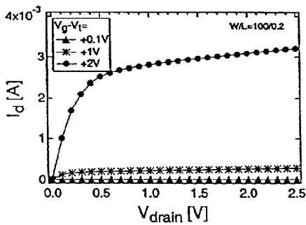
FIG 13 Output characteristics of a 0.2µm aerosol-nanocrystal floating-gate MOSFET; drive current = 30µA/µm.
