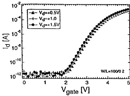
FIG 12 ... Subthreshold characteristics of a 0.2µm n-type aerosol-nanocrystal floating-gate MOSFET (subthreshold slope = 200mV/dec; DIBL = 100mV/V).
