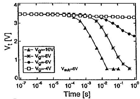
FIG 15 Erase transients (uniform FN tunneling).
