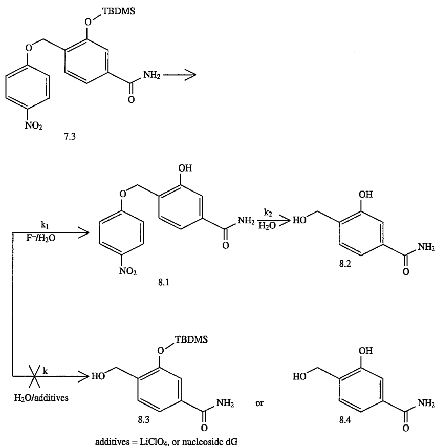
SCHEME 8
