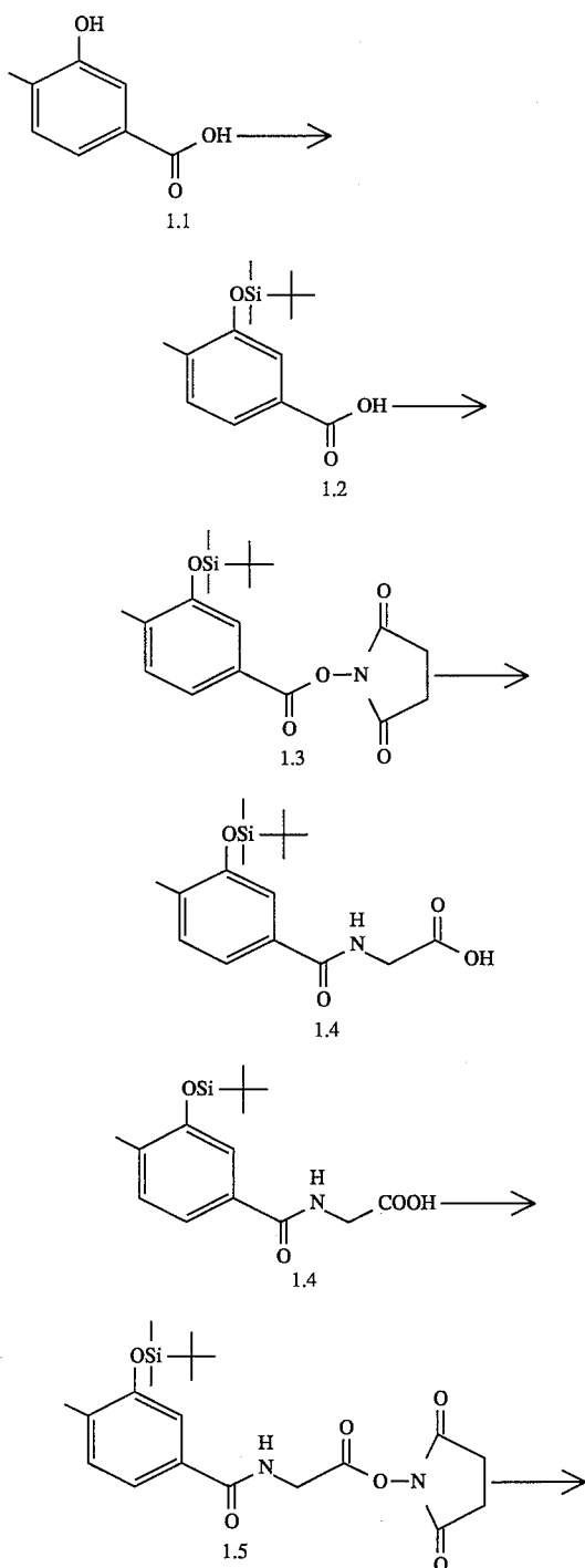
SCHEME 1
