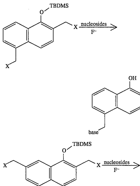
SCHEME 10
