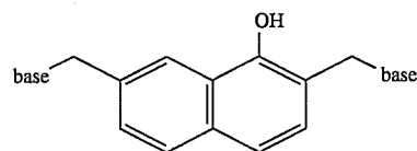
-continued SCHEME 10
