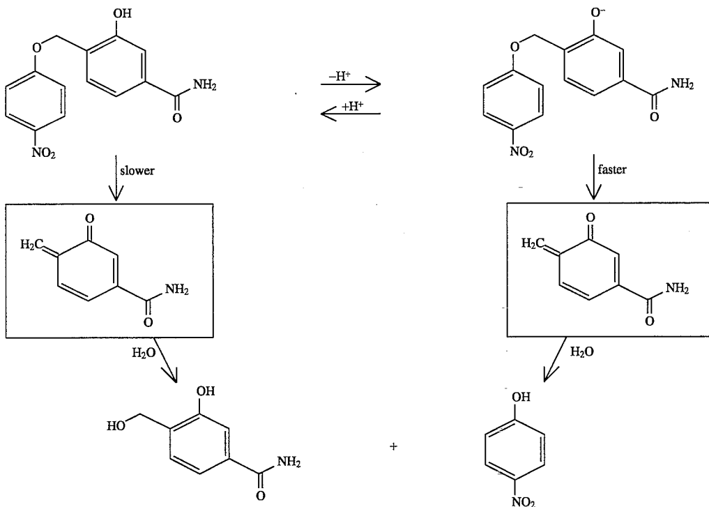
SCHEME 9
