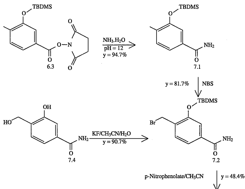
SCHEME 7
