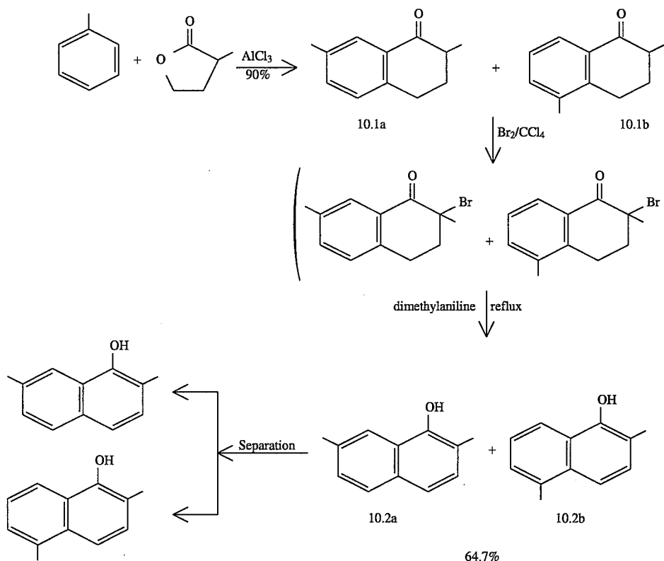
SCHEME 11
