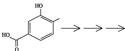
SCHEME A
