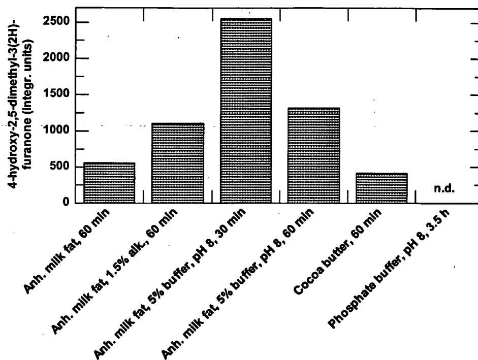
Figure 1: Effect of reaction medium on 4-hydroxy-2,5-dimethyl-3(2H)-furanone accumulation in rhamnose/proline fat-based reaction flavours.
