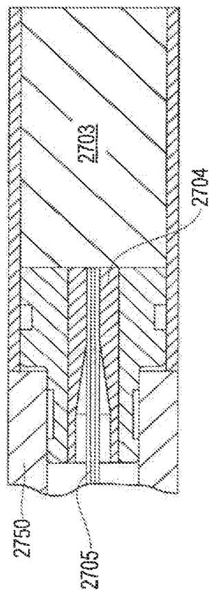
Z-Y SECTION FIG. 27C
