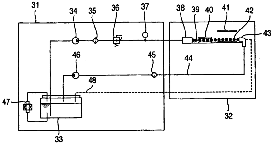
FIG.7 PRIOR ART
