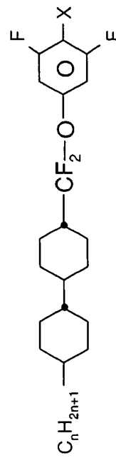
CCQU-n-X (X = F, Cl, "OT" = OCF 3 , "OD" = OCF 2 H)
