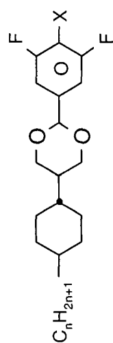
CDU-n-X (X = F, Cl, "OT" = OCF 3 , "OD" = OCF 2 H)
