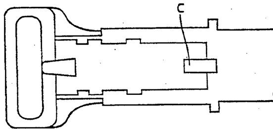
FIG. 19 (PRIOR ART)
