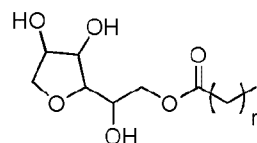
Sorbitan Laurate ( n = 10 )
