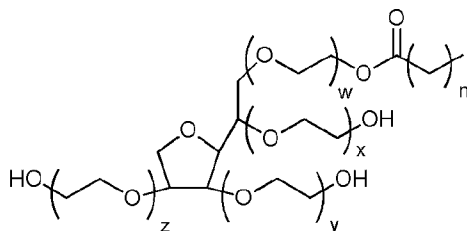
Polyoxyethylene Derivative of a Sorbitan Ester
